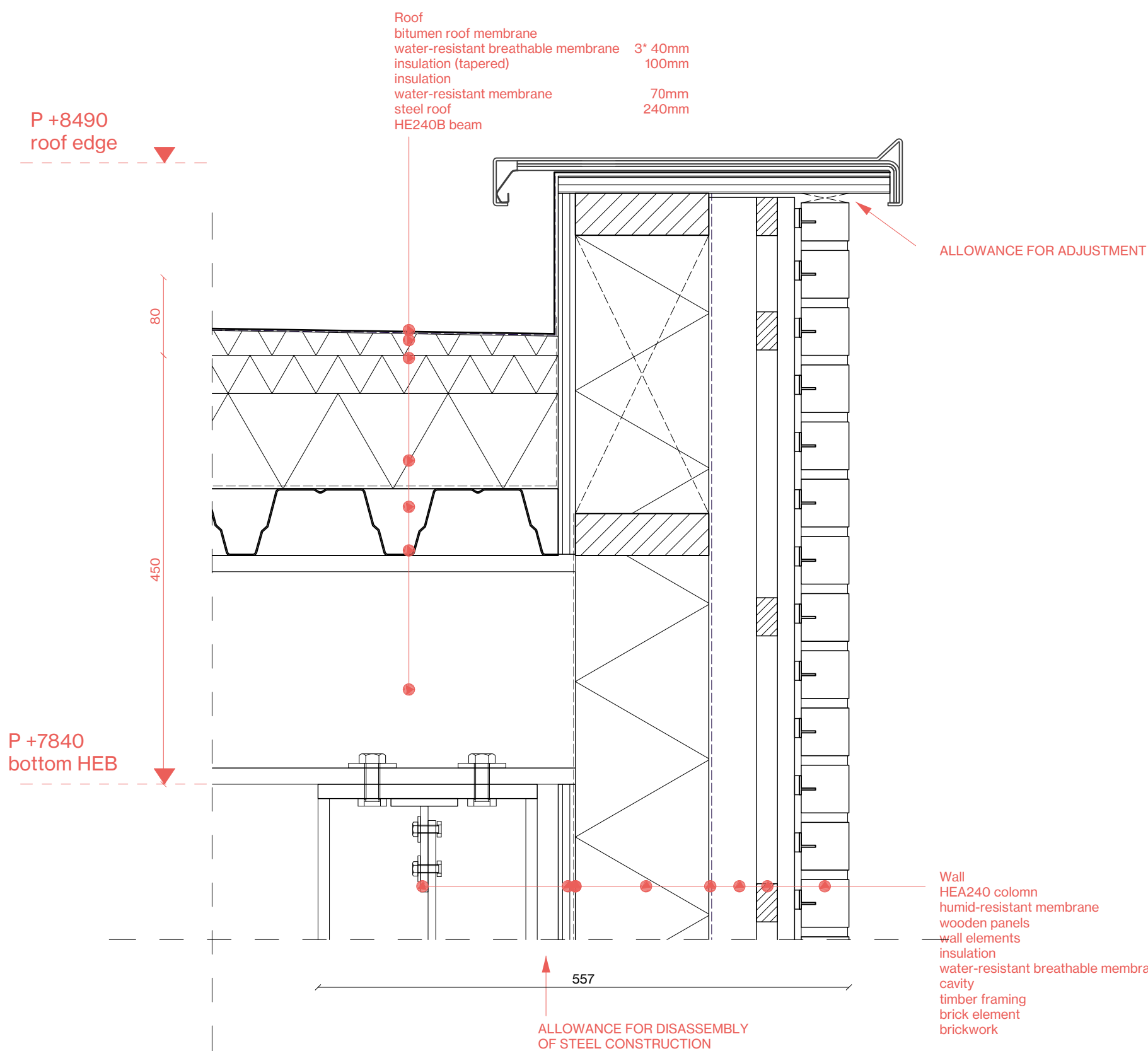
DETAIL 1:5 - D
