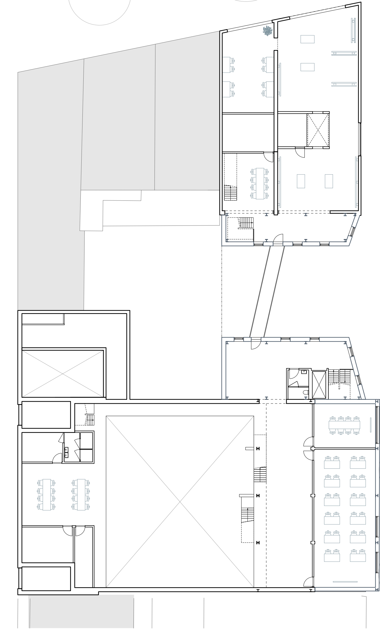
FIRST FLOOR 1:200
