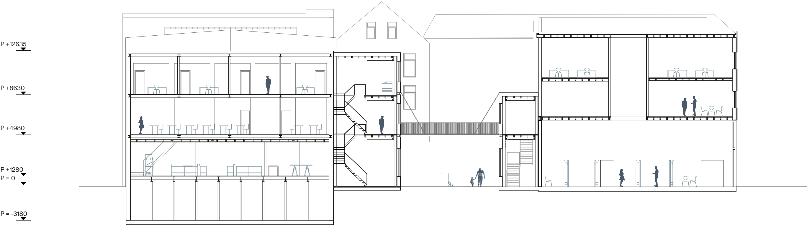
SECTION AA' 1:200
