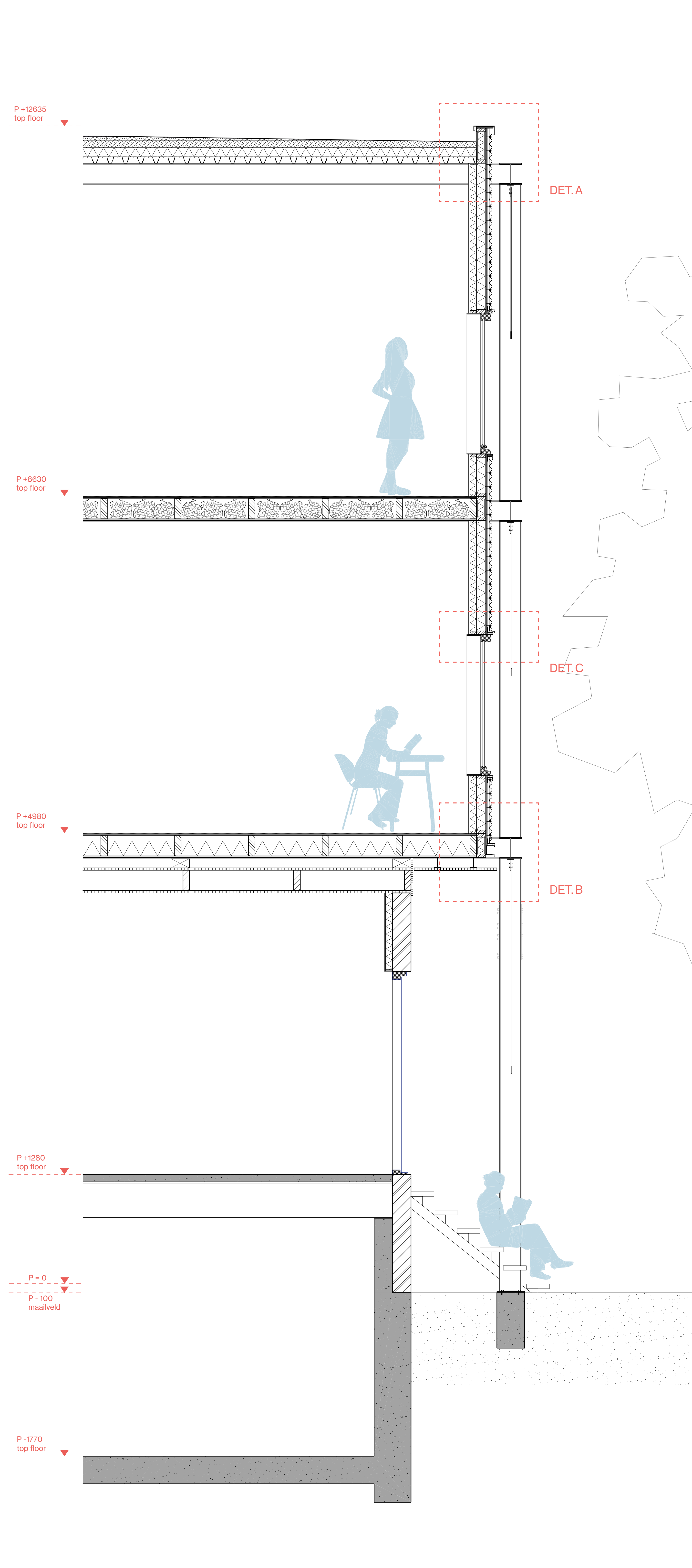
FRAGMENT 1:20 - A
