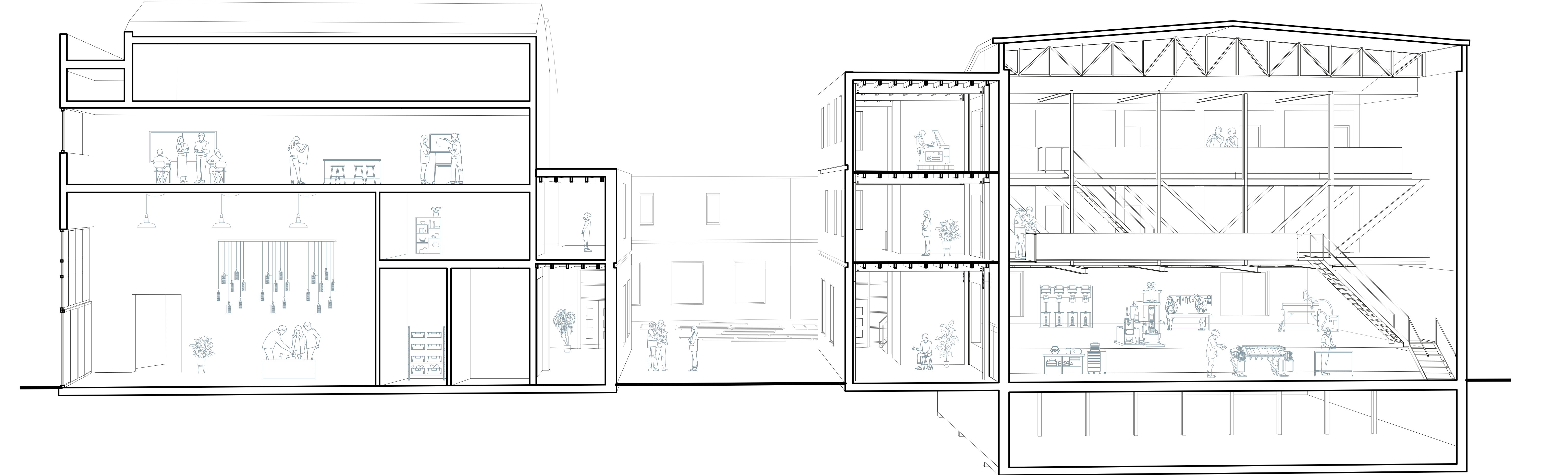
SECTION AA' 1:200
