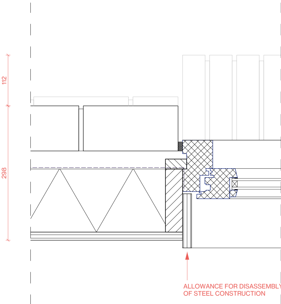
DETAIL 1:5 - F
