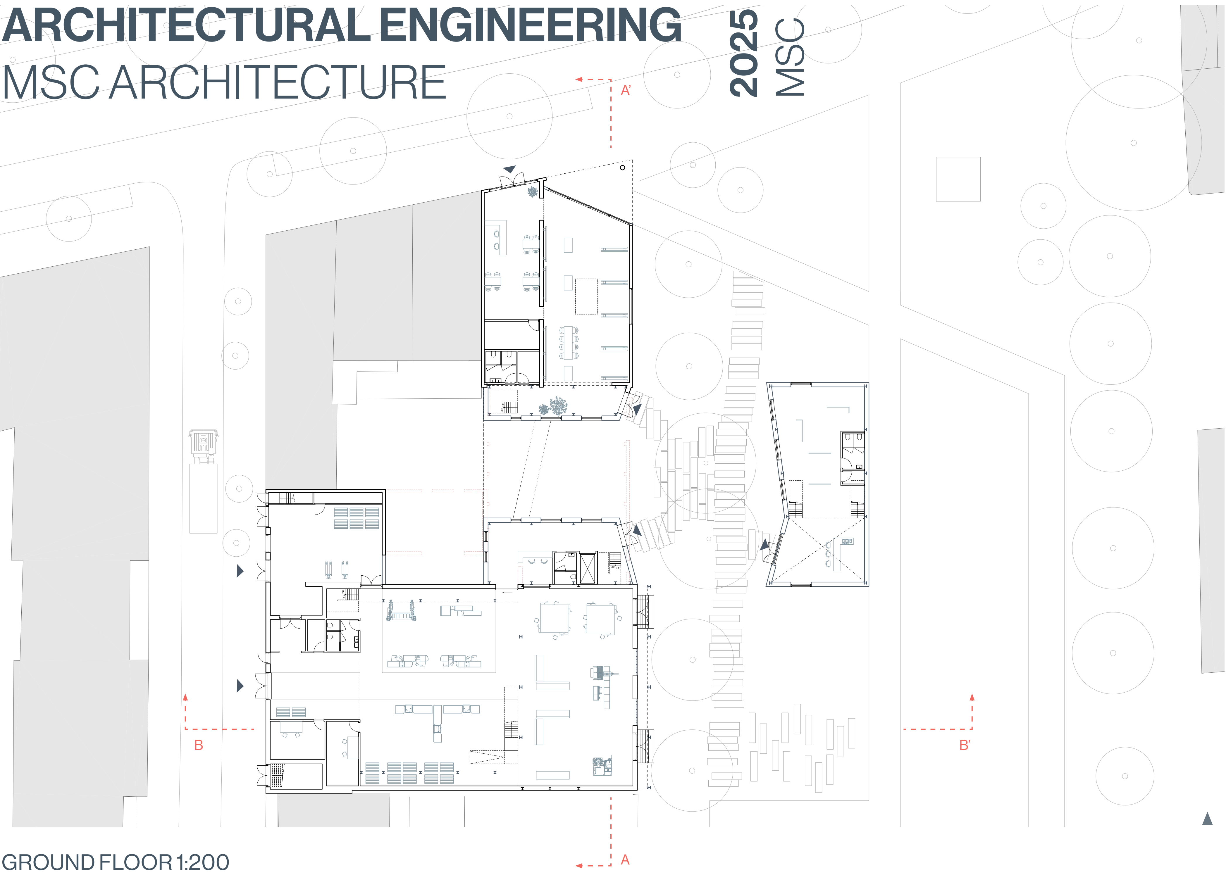
GROUND FLOOR 1:200
