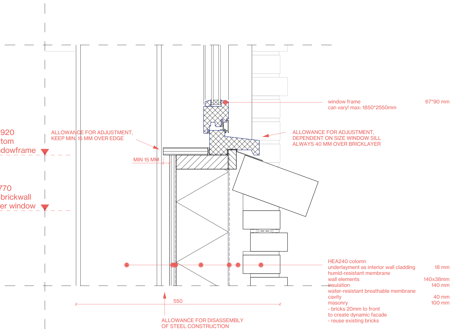
DETAIL 1:5 - E
