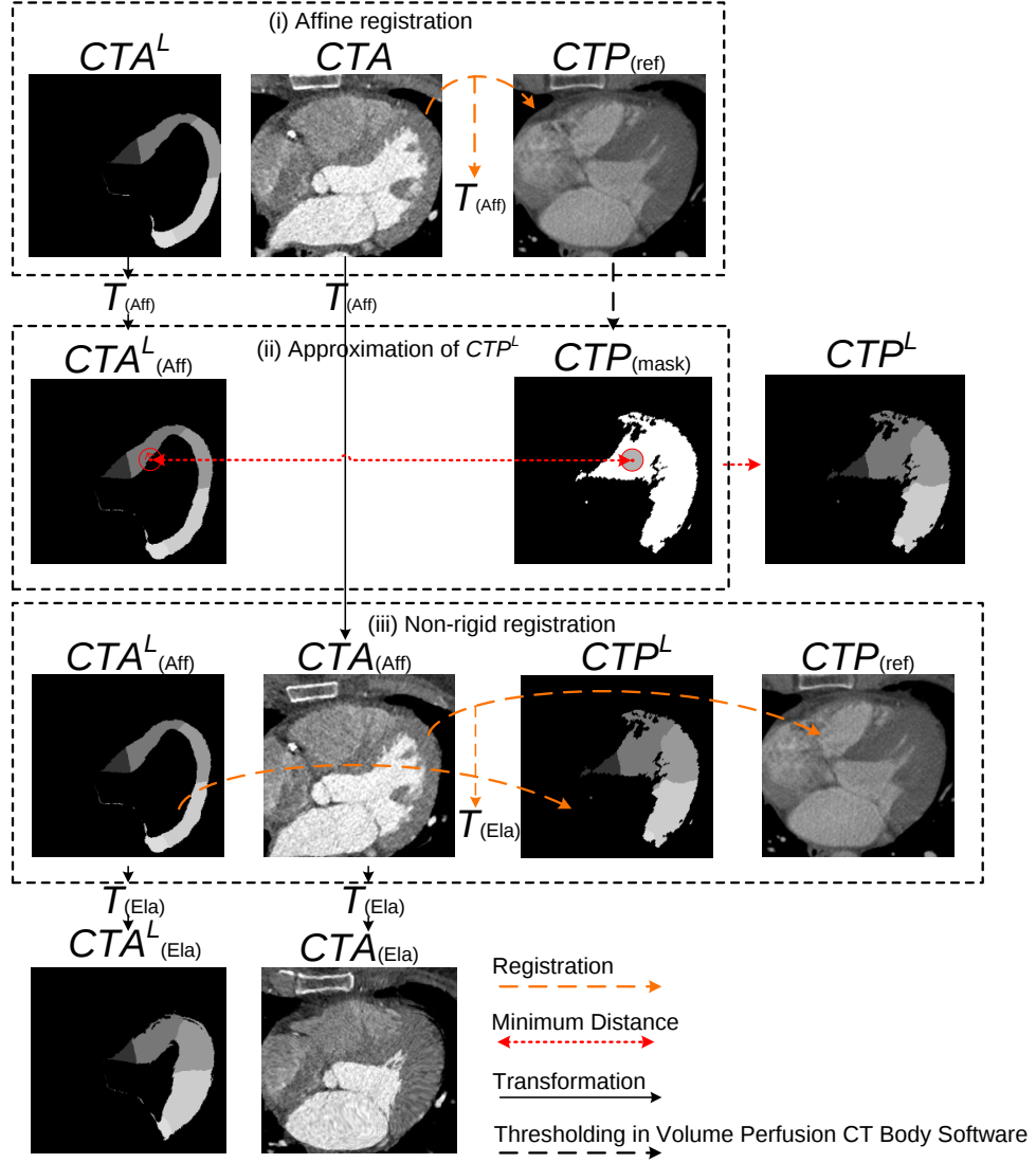
FIG. 4. Workflow for the registration of CTA to CTP_{(ref)} . CTA^L is formed by assigning to each CTA^{L_k} its index k and merging them in one image. i) Affine registration of CTA to CTP_{(ref)} . ii) Approximation of myocardial territories CTP^L by minimum distance to the CTA^L_{(Aff)} s. iii) Non-rigid registration of CTA_{(Aff)} and CTA^L_{(Aff)} to CTP_{(ref)} and CTP^L . CTA^L_{(Aff)} , CTP^L and CTA^L_{(Ela)} are formed similarly as CTA^L by merging the respective myocardial territories.
