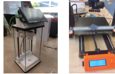
Fig. 11. 3 rd design iteration with Raspberri pi and development of dedicated 3D Printer.
