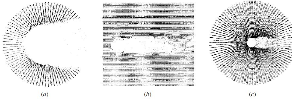
Figure 22. Construction of velocity field for pressure evaluation. (a) Near field, (b) far field and (c) combined velocity field (Fujisawa et al., 2005).
