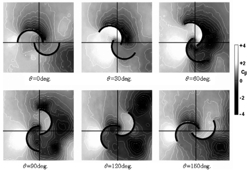
Figure 26. Pressure distributions around a Savonius rotor (Murai et al. 2007). Pressure distribution for various angles of attack at a tip speed ratio of 0.5.
