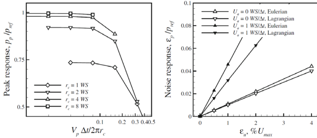
Figure 9. Simulation of pressure determination for a linearly convected Gaussian vortex; left: Peak pressure response with vortex turnover time, Lagrangian approach; Right: Noise response; V_p and r_c are the vortex peak velocity and core radius, respectively (Kat & Oudheusden, 2012).
