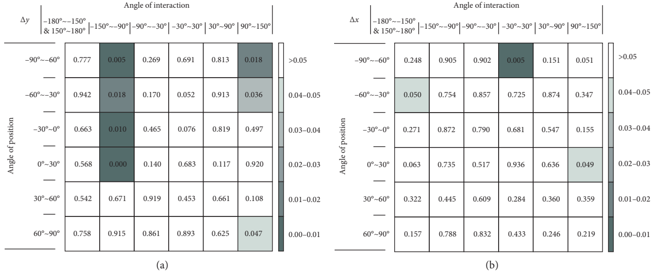
FIGURE 9: The p value of the number of interacting pedestrians with lateral and longitudinal deviations.
