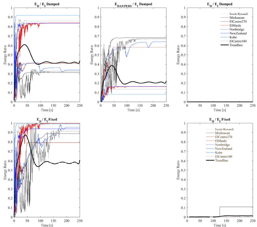
FIGURE 5.16 Energy ratios of the outrigger systems under small earthquake levels
