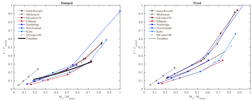
FIGURE 5.32 Normalized column stress ( \sigma/\sigma_{yield} ) to normalized overturning moment ( M\theta/M\theta_{max} ) of the studied outrigger configurations subjected to four earthquake levels of all ground motions.
