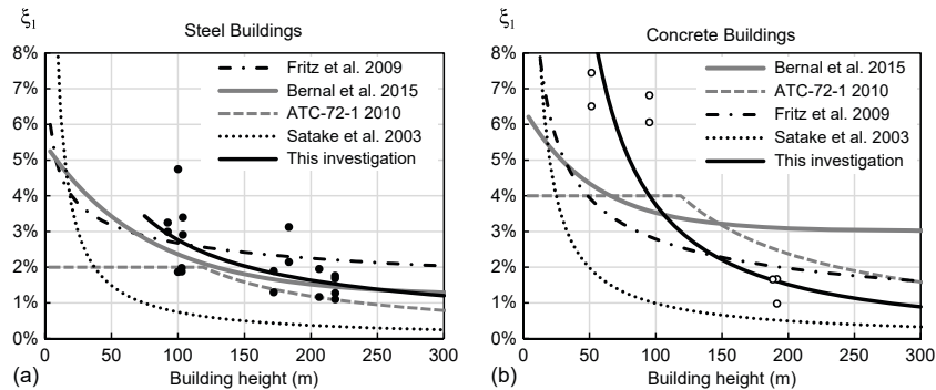
FIGURE 2.6 Identified damping ratios for the fundamental mode versus building height, compared to some proposed recommendations: (a) steel buildings; (b) reinforced concrete buildings. Image source: Cruz and Miranda, 2017 - With permission from ASCE
