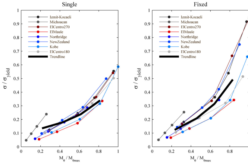
FIGURE 7.3 Normalized column stress ( \sigma/\sigma_{yield} ) to normalized overturning moment ( M_{\theta}/M_{\theta_{max}} ) of the studied outrigger configurations subjected to four earthquake levels of all ground motions.
