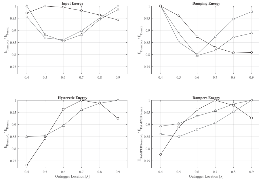
FIGURE 4.23 Normalized (actual/maximum) energy distributions of the outrigger structure ( \zeta=2\% - C_d=1.18E+05\text{kN-s/m} ) according to outrigger location ( \lambda=0.4 - 0.9 ) under four intensity levels of 1940 El Centro earthquake.
