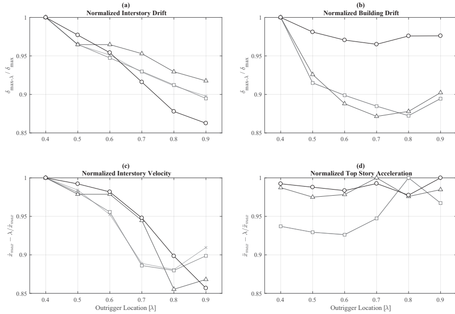
FIGURE 4.21 Normalized (actual/peak) drift, velocity and lateral accelerations for different outrigger locations ( \lambda = 0.4 - 0.9 ), of the damped outrigger building ( \zeta = 2\% , C_d = 1.18E+05 \text{ kN-s/m} ) subjected to four intensity levels of 1940 El Centro earthquake
