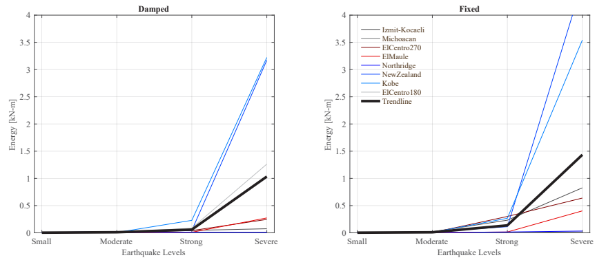
FIGURE 5.24 Damping energy dissipated by the outrigger in the damped (left) and fixed (right) system
