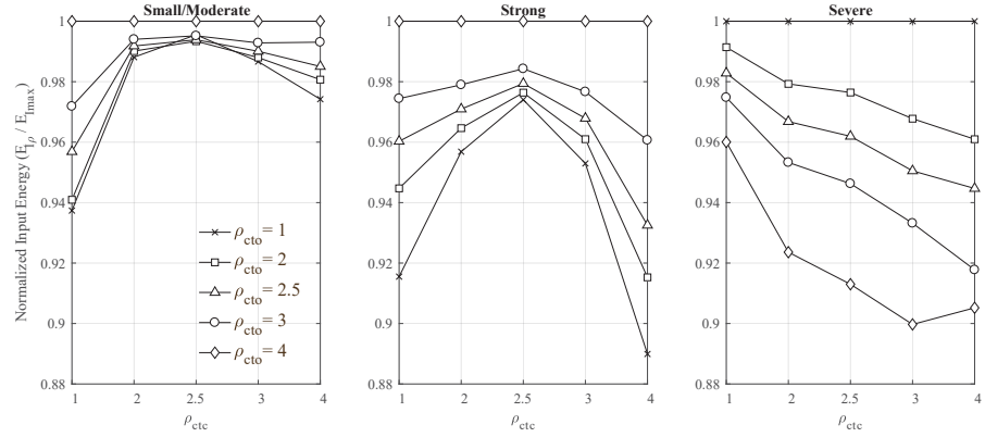
FIGURE 4.31 Variations of the Normalized Input Energy ( E_p/E_{max} ), according to combined effect of \rho_{cto} and \rho_{ctc} under different earthquake levels of 1940 El Centro earthquake; C_d = 1.18E+05 \text{ kN-s/m} , \lambda = 0.7 and \zeta = 1.5\% .
