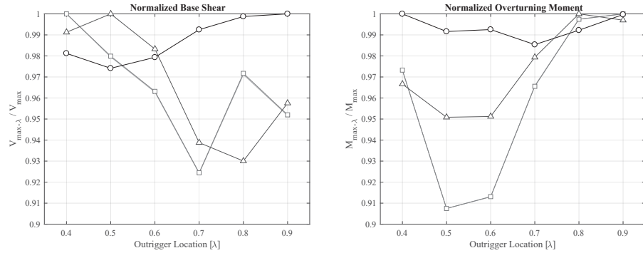
FIGURE 4.22 Normalized (actual/peak) base shear and overturning moments of the damped outrigger building ( \zeta = 2\% , C_d = 1.18E+08 \text{ kN-s/m} ), subjected to four intensity levels of 1940 El Centro earthquake, with different outrigger locations ( \lambda = 0.4 - 0.9 ).
