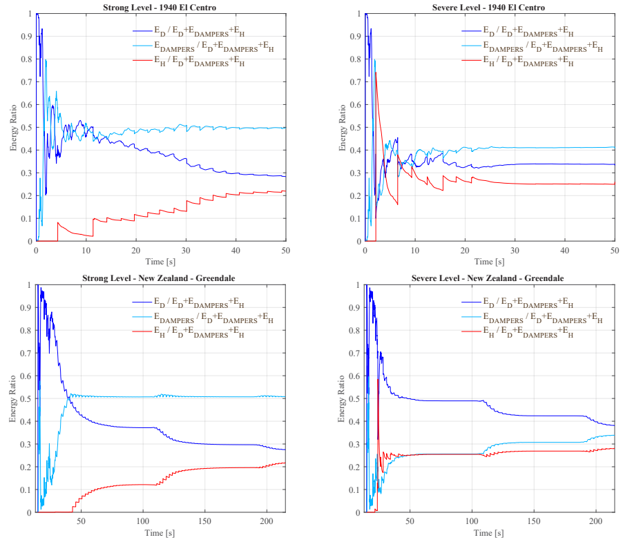
FIGURE 5.36 Energy Ratios of the damped outrigger ( C_d = 1.18 \times 10^5 \text{ kN-s/m} , \lambda = 0.7 and \zeta = 2.0\% ), under strong and severe levels of 1940 El Centro and New Zealand – Greendale earthquakes
