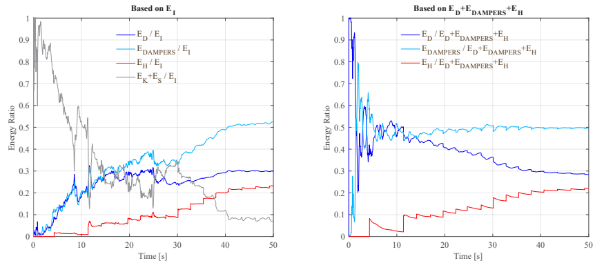
FIGURE 5.35 Energy ratios based on E_I and E_D+E_{dampers}+E_H for the damped outrigger under strong earthquake level of 1940 El Centro earthquake; C_d=1.18E+05\text{kN}\cdot\text{s/m} , \lambda=0.7 and \zeta=2.0\% .
