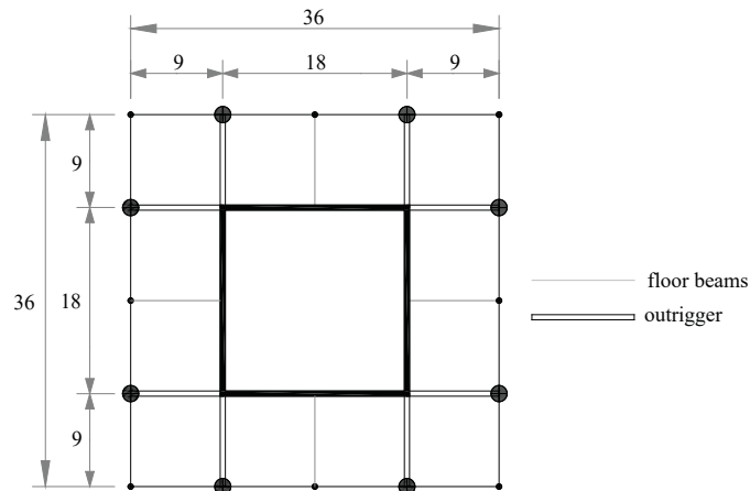
FIGURE 4.1 36m square building plan, based on a 9m grid. Note that the outriggers are not loading all the perimeter columns.
