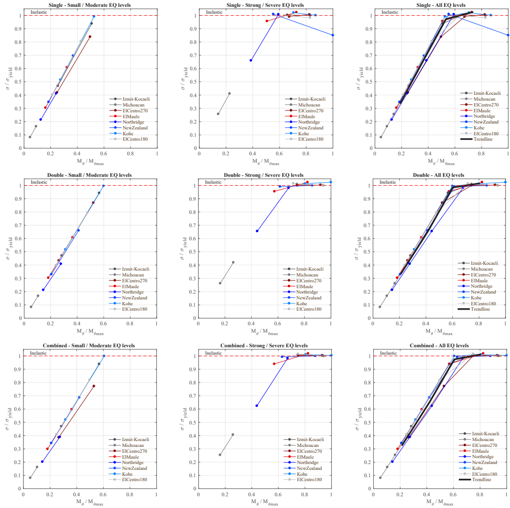
FIGURE 6.16 Normalized core stress ( \sigma/\sigma_{yield} ) to normalized overturning moment ( M_{\theta}/M_{\theta_{max}} ) of the single (upper row), double (middle row) and combined (lower row) outrigger configurations subjected to four earthquake levels of all ground motions.
