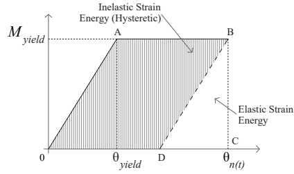
FIGURE 3.6 Strain energy for an inelastic system defined by M - \theta
