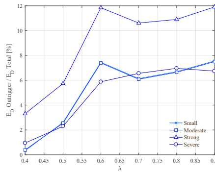
FIGURE 5.23 Damping energy (in %) dissipated only by the outriggers, under the combined influence of \lambda and different earthquake levels of 1940 El Centro earthquake; C_d = 1.18E+05 \text{ kN-s/m} and \zeta = 2.0\% .
