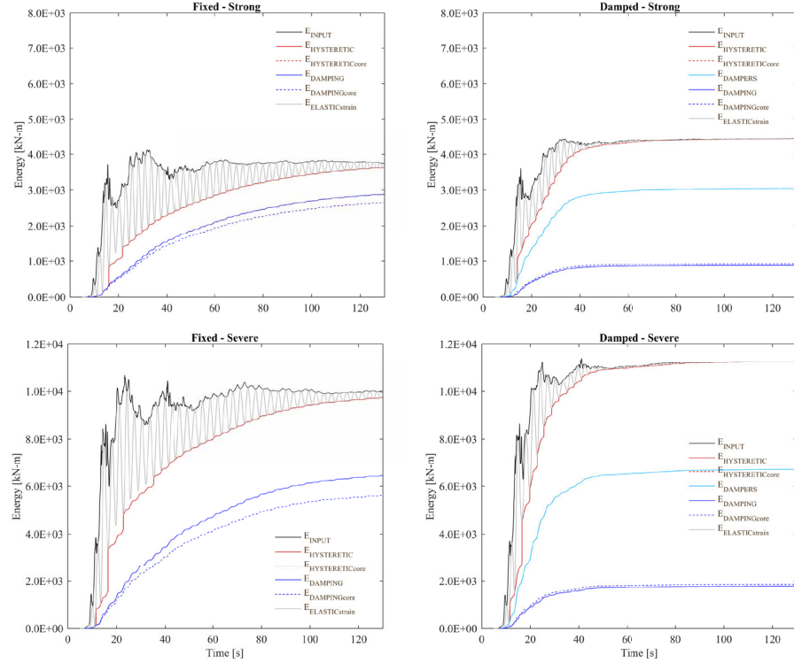
FIGURE 5.34 Energy distribution of the fixed and 1.18E+05kN-s/m damped outrigger structures under strong and severe levels of Izmit-Kocaeli earthquake ( \lambda=0.7 and \zeta=2.0\% ).
