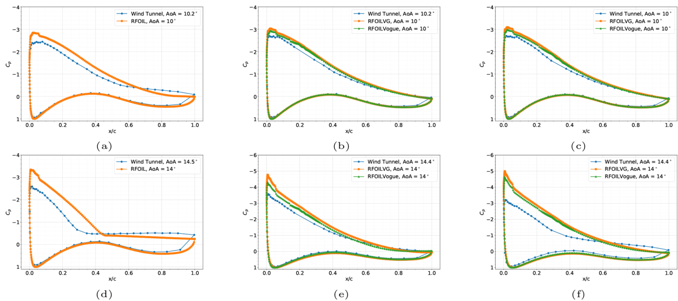
Figure 17. Chordwise pressure distributions at AoA 10° (top row) and AoA 14° (bottom row) with adverse pressure gradients for the FFA-W3-241 airfoil with forced transition using ZZ tape at a Reynolds number of 1.6 million with no VGs (a, d), 4 mm VGs placed at 20 % chord (b, e), and 6 mm VGs placed at 30 % chord (c, f) placed on the upper surface. Wind tunnel C_p data are digitised from Fuglsang et al. (1998).
