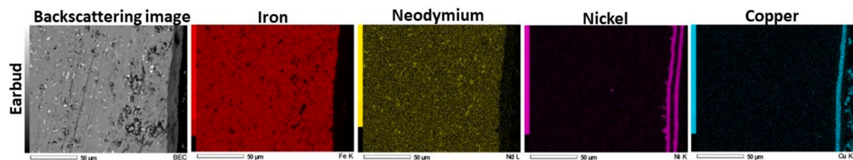
Fig. 5. Scanning backscattered image and EDS elemental mapping of the cross section of the NdFeB permanent magnet sample from earbud for Fe, Nd, Ni and Cu.
