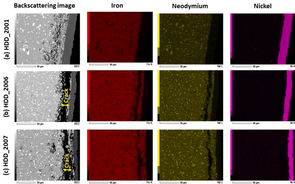
Fig. 4. Scanning backscattered images and EDS elemental mappings for Fe, Nd and Ni in the cross section of different end-of-life NdFeB permanent magnets from hard-disc drivers produced in different years: (a) 2001; (b) 2006; (c) 2007.
