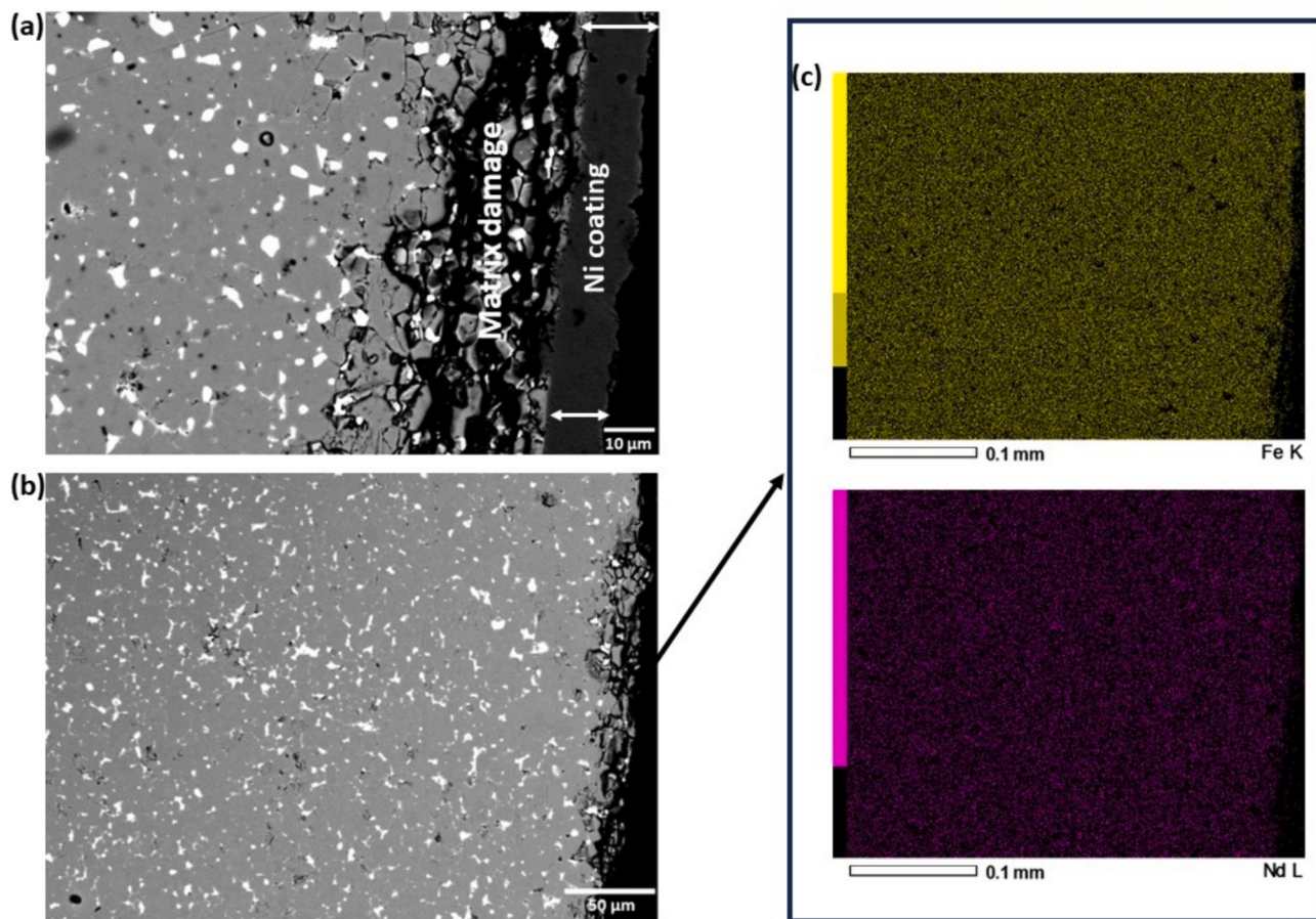
Fig. 8. Scanning backscattered images from the cross-sections of NdFeB PMs after de-coating in 5 M \text{NH}_3 + 0.25 M \text{NH}_4\text{Cl} at 75 °C: (a) Ni-coated PM sample from HDD; (b) Zn-coated PM sample from E-scooter; (c) EDS mapping of Fe and Nd for the cross-section image (b).
