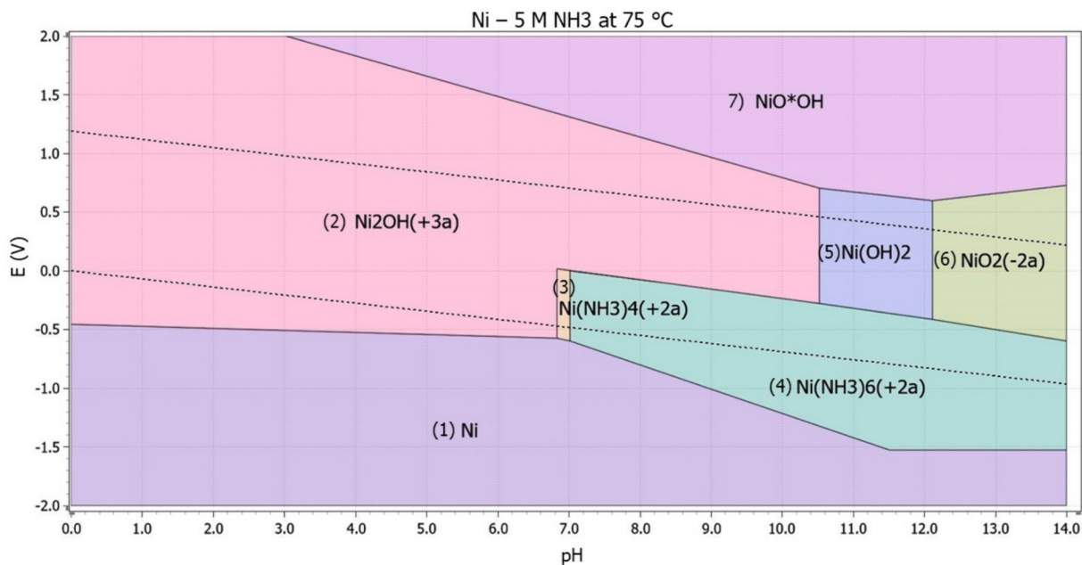
Fig. 9. E-pH diagram of Ni-NH 3 at 75 °C, considering 5 M \text{NH}_3 and Ni activity of 10^{-6} M.
