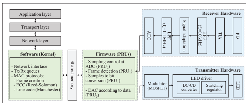
FIGURE 3. Diagram of the front-end transceiver and the communication stack of OpenVLC 1.4.
