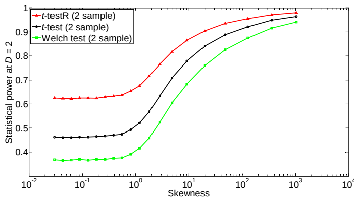
Figure 3. Statistical power at D = 2 of the two-sample t -test, the two-sample t -test after rank transformation ( t -testR), and the Welch test, as a function of the degree of skewness of the lognormal distribution ( N = M = 3 ).
