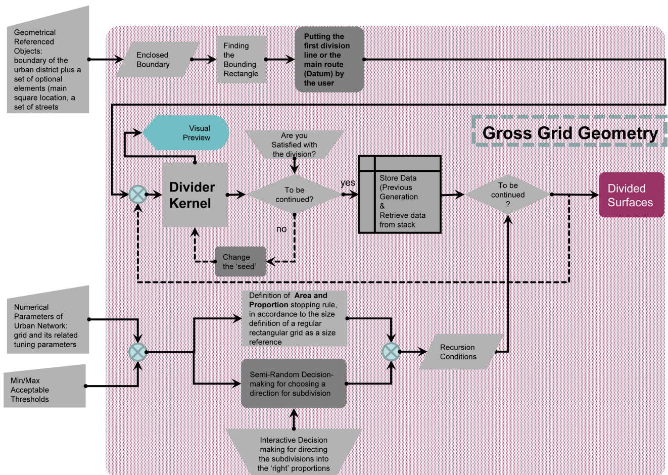
Figure 4 - Flowchart of the recursive street network generator.
