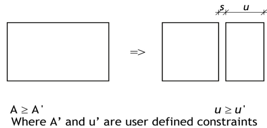
Figure 2 - Recursive rule
