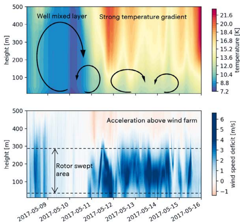
▲ FIG. 3: Temperature profile over time (top) and velocity deficit in the middle of the wind farm (bottom).
