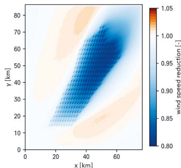
▲ FIG. 4: Composite plot for all south-westerly wind directions of the velocity deficit.
