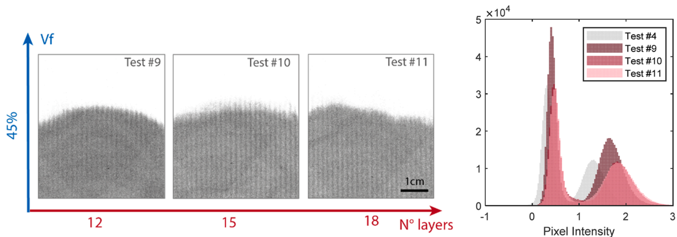
Fig. 9. Comparison of scattering images obtained for tests #9, #10 and #11 with the corresponding histograms which are compared to the one of test #4. The scale is the same for all pictures.
