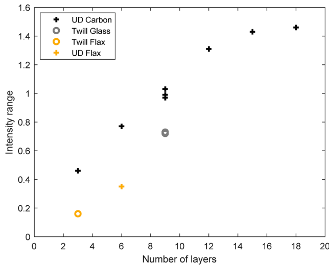
Fig. 10. Intensity range of scattering images versus the fabric number of layers.
