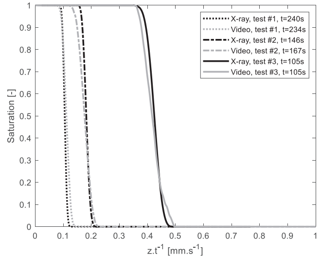
Fig. 6. Comparison of S(z, t) curves built from optical and X-ray acquisitions.
