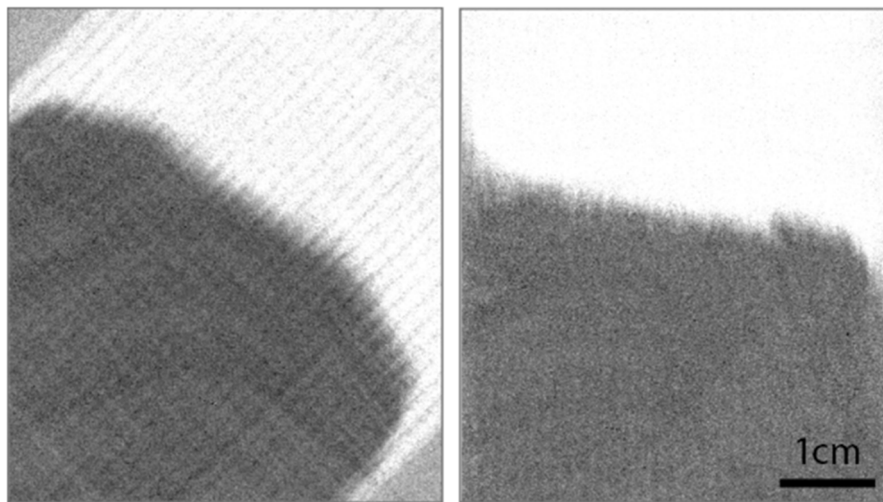
Fig. 11. Scattering image resulting of rotating the setup 45° (test #15) compared to the scattering image of test #4.
