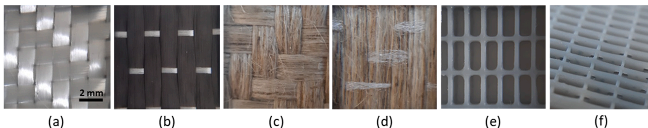
Fig. 1. Porous media: (a) twill glass, (b) UD carbon, (c) twill flax, (d) UD flax fabrics, (e) top and (f) side view of the 3D printed structure. The scale is the same for all pictures.
