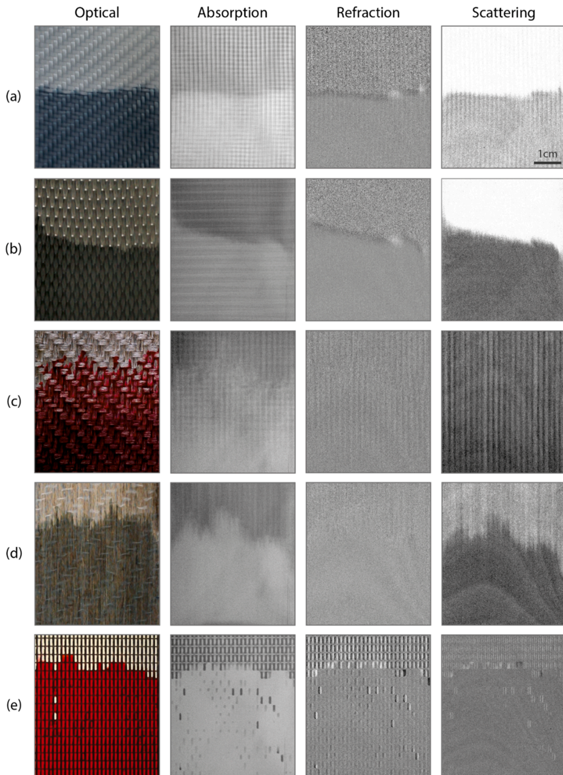
Fig. 4. Example of flow patterns observed in optical, absorption, refraction and scattering images obtained for the different reinforcements (a) Twill Glass (test #2), (b) UD Carbon (test #4), (c) Twill Flax (test #12), (d) UD Flax (test #13) fabrics and (e) the 3D printed structure (test #14). The image of the optical view does not correspond to the flow shown in X-ray images as the X-ray infrastructure did not allow capturing videos during X-ray measurements. The scale is the same for all pictures.
