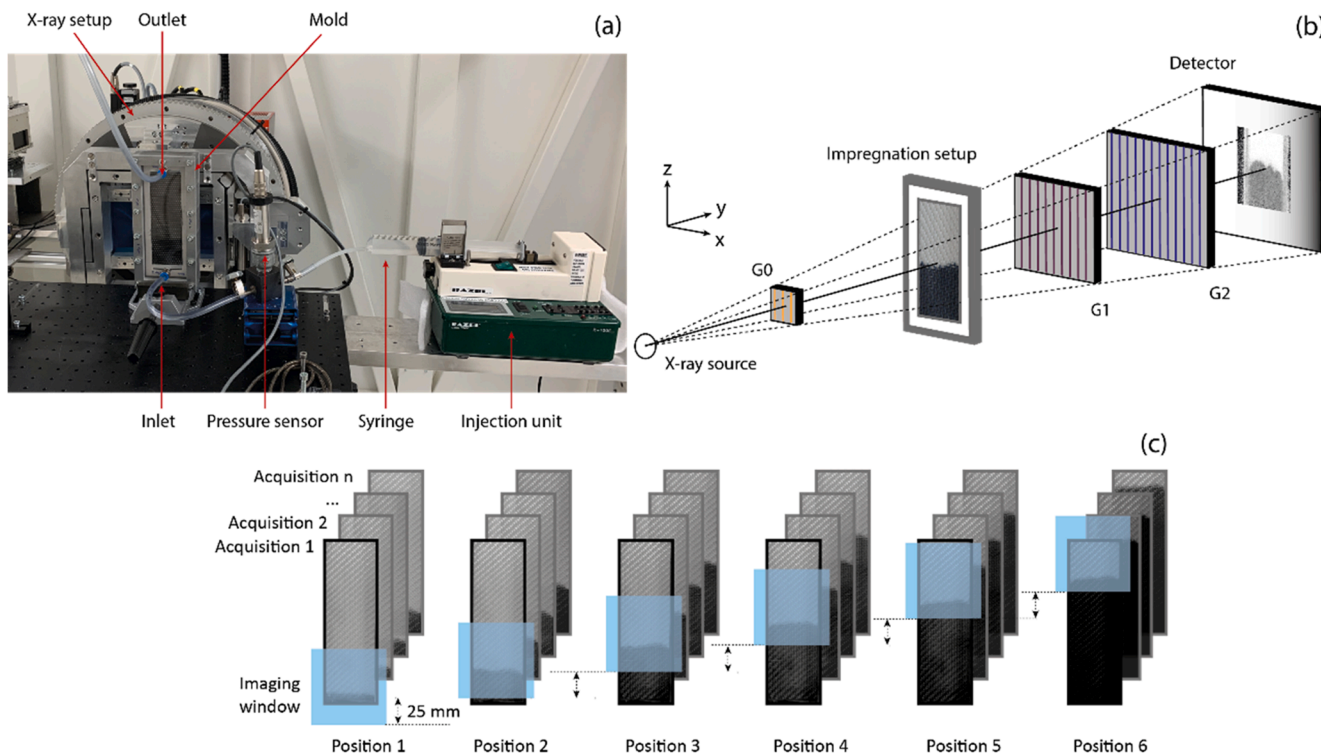
Fig. 2. (a) Impregnation setup, (b) schematic of the X-ray phase contrast imaging system and (c) illustration depicting the flow acquisition procedure.
