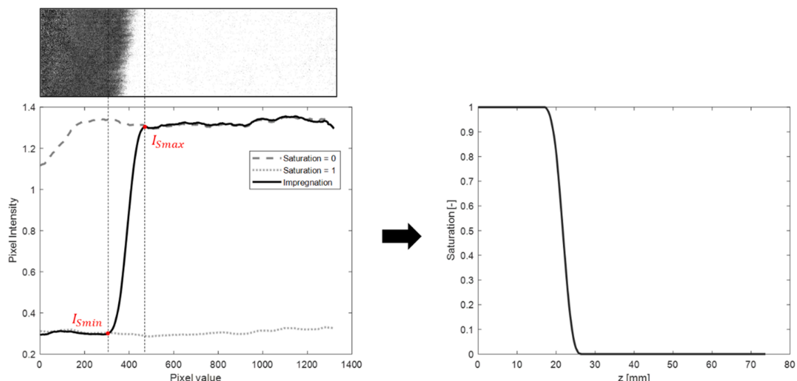
Fig. 3. Methodology for the construction of S(z) curve from the grayscale scattering image (example taken from an acquisition of test #4).
