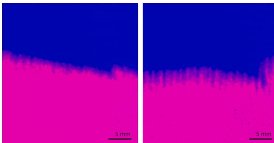
Fig. 12. Superimposed absorption and scattering images for visualization of flow patterns. Acquisition corresponding to test #4 (left) and test #16 (right).
