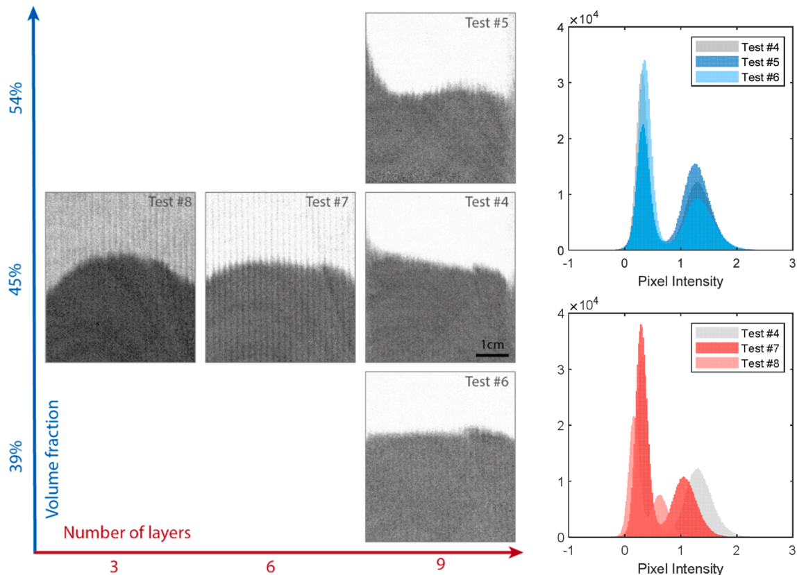
Fig. 8. Comparison of scattering images obtained for the different impregnation configurations of the carbon fabric with the corresponding histograms. The scale is the same for all pictures.
