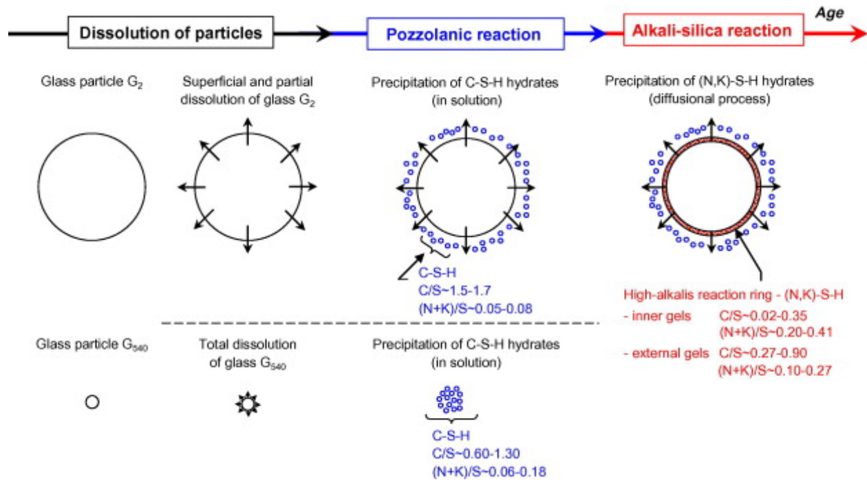
Figure 4. Schematic representation showing successive reactions of coarse and fine glass particles in the cementitious matrix (Idir et al., 2011)
