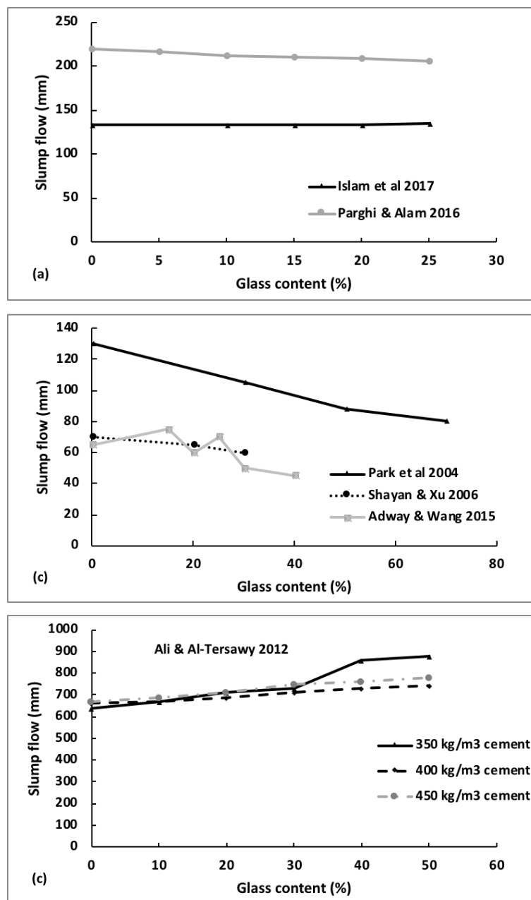
Figure 1. Influence of waste recycled glass on slump behaviour of (a) mortar, (b) concrete and (c) SCC using glass powder (Adaway and Wang, 2015; Ali and Al-Tersawy, 2012; Islam et al., 2017; Parghi and Alam, 2016; Park et al., 2004; Shayan and Xu, 2006).
