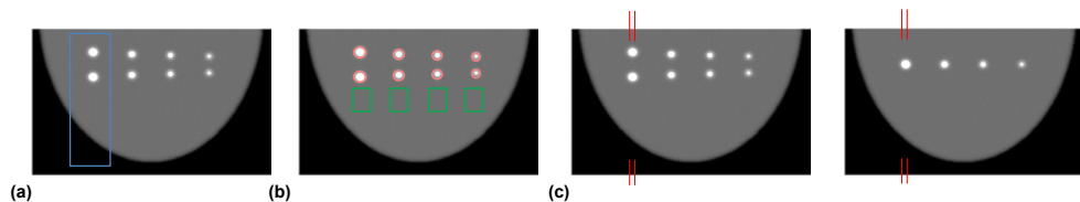
Figure 2-4 Slices through the breast phantom with regions used in analysis indicated. (a) Region used in Focusing Mode for imaging largest spheres. (b) Red circles are regions for contrast and CNR calculation, green box is background region for the same. (c) Lines indicate location of profiles shown in Figure 2-8.
