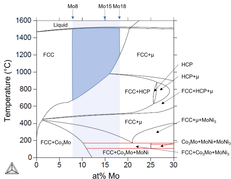
Fig. 1. Equilibrium pseudo-binary phase diagram of the (CoNi) 100-x Mo x alloy system ( x = 0 –30 at%) in the temperature range of 0–1600°C. The composition range from (CoNi) 92 Mo 8 to (CoNi) 82 Mo 18 is highlighted in blue color.
