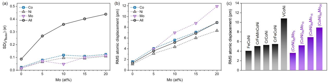
Fig. 9. Ab initio calculations for the lattice distortion of the (CoNi) 100-x Mo x system ( x = 0 –20 at%). (a) Standard deviation (SD) of the Bader charges and (b) RMS displacements of alloys as a function of the Mo content. The solid black lines show the values for all the elements, whereas the dotted blue, gray, and purple lines show the values of Co, Ni, and Mo, respectively. (c) The RMS displacement for various FCC CCAs [8].
