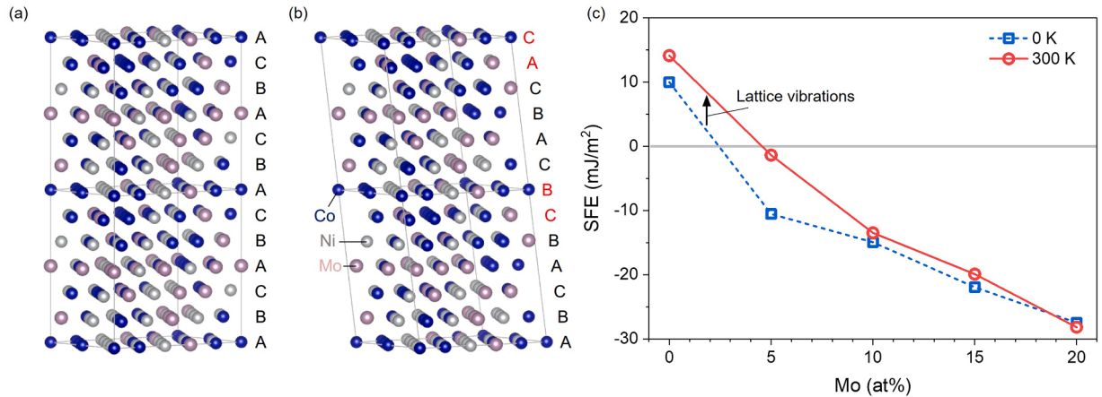
Fig. 10. Ab initio calculations for the SFE of the (CoNi) 100-x Mo x system ( x = 0 –20 at%). Example for supercell models of chemically disordered FCC (CoNi) 80 Mo 20 alloy (a) without SFs and (b) with a SF obtained by the tilted-supercell approach. Labels A, B, and C correspond to the stacking sequence of the {111} planes, and the interlayer spaces sandwiched by the red labels to the SFs. The simulation cells are repeated twice along the \langle 111 \rangle direction to better visualize the tilted-supercell approach. (c) Ab initio SFEs of the alloys as a function of the Mo content. The dashed blue and the solid red lines show the results at 0 K and at 300 K with the contributions of lattice vibrations, respectively.
