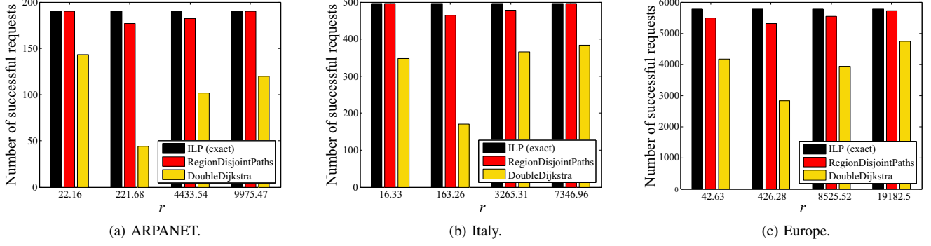
Fig. 12: Number of successful requests. All pairs of nodes are requests. Variable r reflects the radius of failure.
