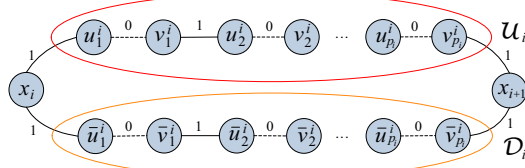
Fig. 5: Lobe of x_i .
