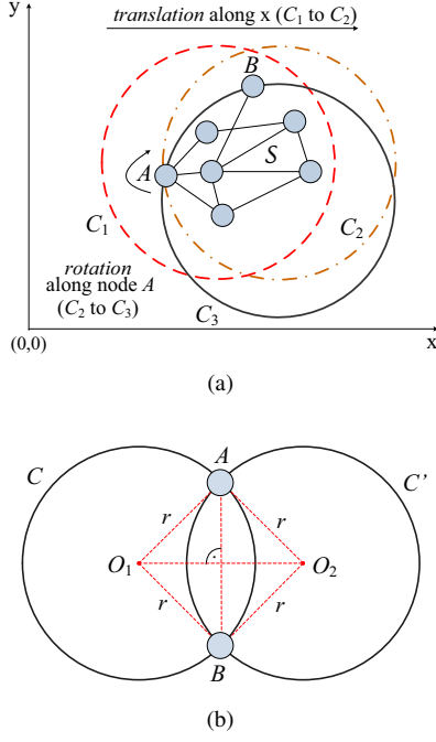
Fig. 3: (a) Visualization of (the proof of) Lemma 1. (b) Possible circles with radius r through nodes A and B .
