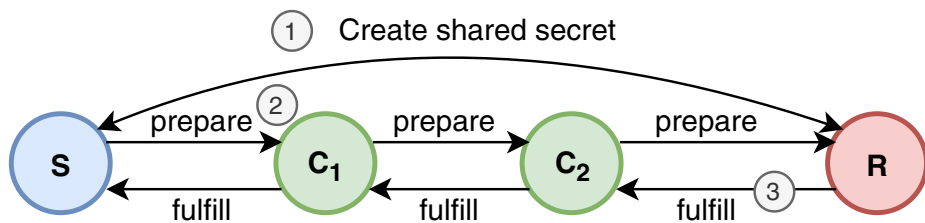
Figure 3 A successful ILPv4 payment from a sender S to a receiver R , using two connectors C_1 and C_2
