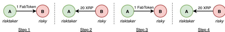
Figure 5 An asset exchange with k = 2 between Alice (A) and Bob (B), trading a total of 2 FabTokens and 40 XRP. During this trade, Alice is the risktaker since she is exposed to counterparty risk. Bob is the risky party since he is able to commit counterparty fraud after step 1 and 3
