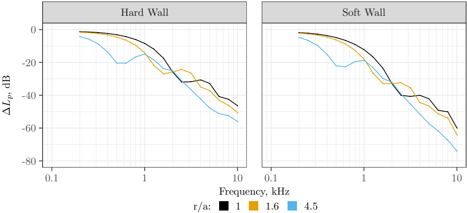
Figure 3.10: Soft-wall model with melamine foam compared to the hard-walled case. The cavity depths are constant with D = 0.01 \text{ m} .
