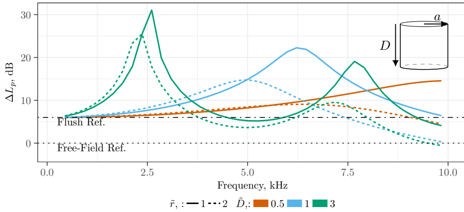
Figure 5.8: Simulated \Delta L_p values with respect to the free-field for different normalized cylindrical cavity depths ( \tilde{D} = D/0.01 m) and radii ( \tilde{r} = a/0.005 m). The solid lines represent the responses for a = 0.005 m. The dashed lines represent the responses for a = 0.01 m. The horizontal dash-dotted and dotted lines represent the flush and free-field responses, respectively. The cavities feature hard walls with no stainless steel cloth covering.
