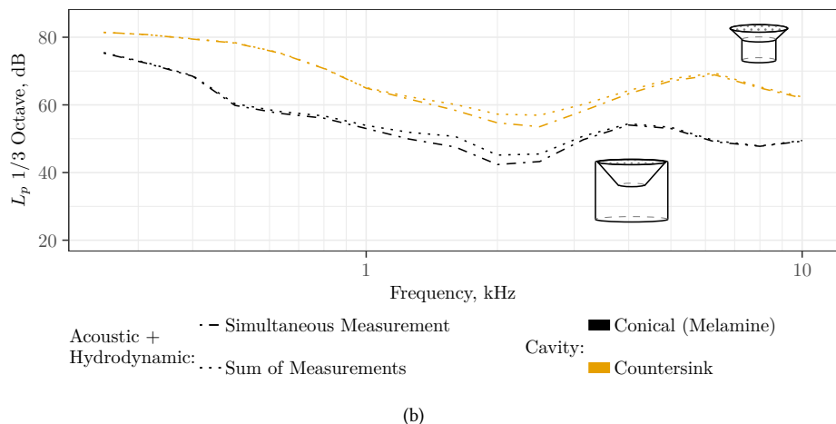
Figure 5.7: a) Independent cavity microphone measurements with only an acoustic source and with only the TBL ( U_\infty = 20 \text{ ms}^{-1} ) present over two cavities. b) Comparison of the measurement of the acoustic source with the TBL present and the sum of the independent measurements.
