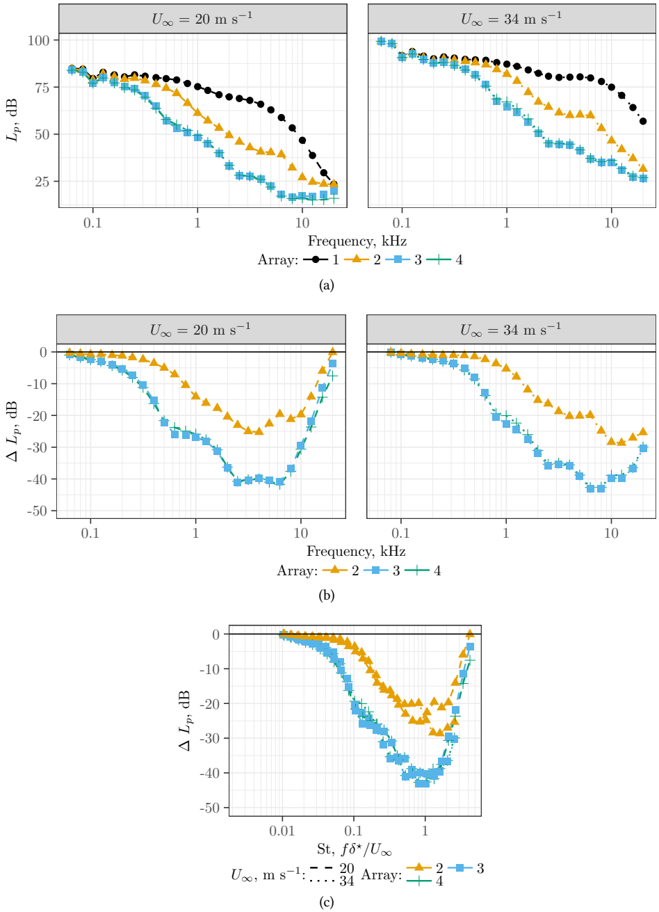
Figure 7.4: Relative increase in the attenuation of TBL spectral energy of the averages over 16 microphones for arrays 1, 2, 3 and 4 for U_\infty = 20 \text{ m s}^{-1} and 34 \text{ m s}^{-1} . a) Measured TBL spectra, absolute frequencies, b) Change in spectra with respect to array 1, absolute frequencies, c) Change in spectra with respect to array 1, non-dimensional frequencies (St).
