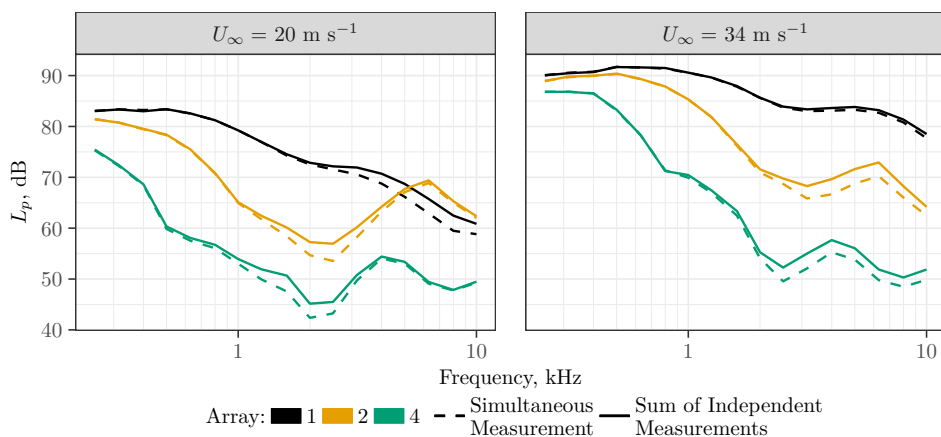
Figure 7.6: Comparison between the single microphone measurement for the case where the TBL was present simultaneously with the acoustic source and the summation of the independently measured TBL only and acoustic source only measurements. The summation of independent measurements was calculated by adding the acoustic powers, i.e., before transforming to the decibel scale. Array 3 is not shown to improve readability.
