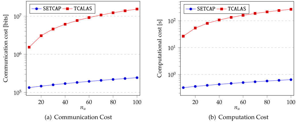
Fig. 6. Comparison between SETCAP and TCALAS [8] in terms of communication (left) and computation (right) costs vs. the number of users.
