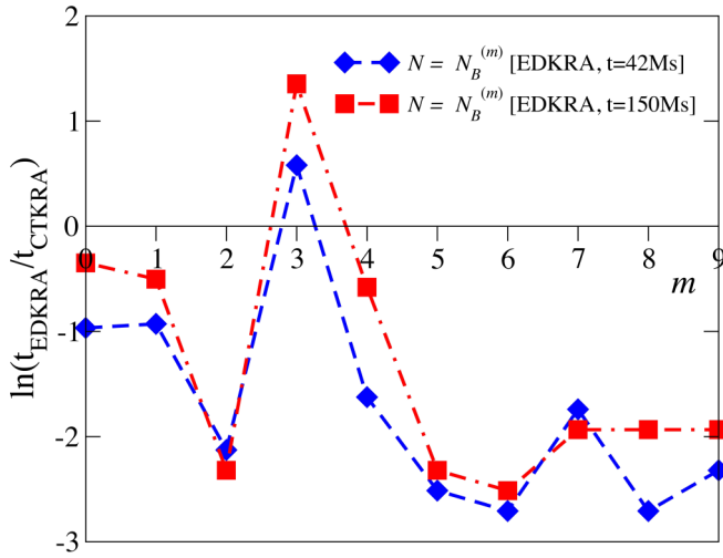
FIG. 7. The ratio of time required for EDKRA and CTKRA reaching the same values of N_B^{(m)} as a function of m after 42 Ms and after 150 Ms have passed with EDKRA kinetics.
