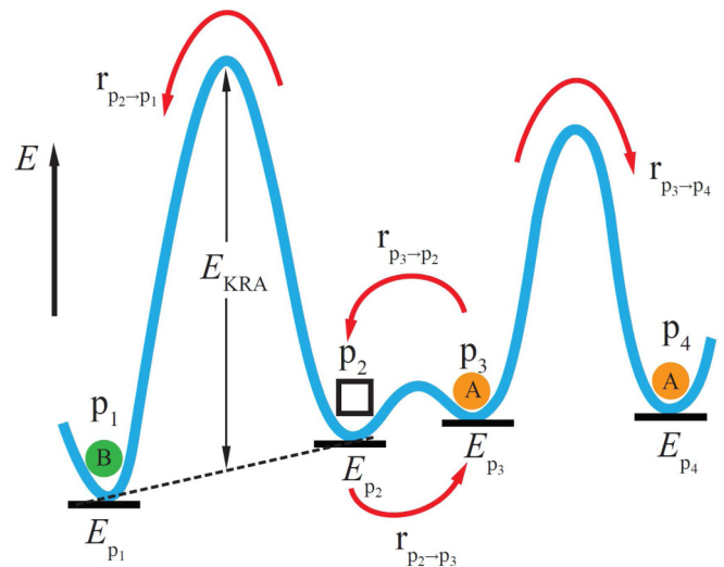
FIG. 3. Schematic diagram of an energy landscape with low barriers between states 2 and 3. Black square represents a vacancy, species C, while orange and green solid circles refer to atomic species A and B.
