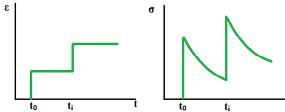
Figure 3.2 Step strain and the corresponding stress response
