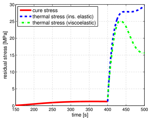
Figure 5.14 Cure and thermal induced stress profile for 160°C molding
