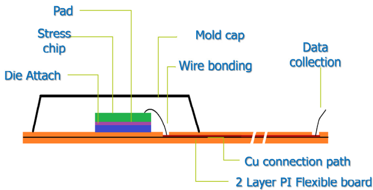
Fig 7.3 Schematic of the designed board and the interconnection
