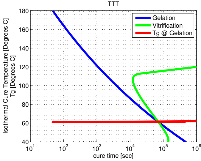
Figure 2.18 Time-Temperature Transformation of the tested Epoxy Compound
