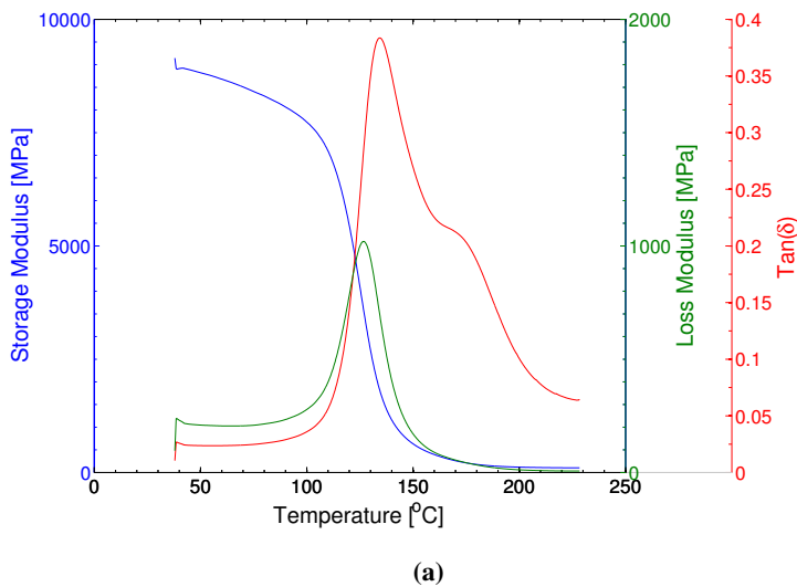
Figure 3.16 DMA temperature scan of a cured Hitachi (a) and Sumitomo (b) samples at 1Hz
