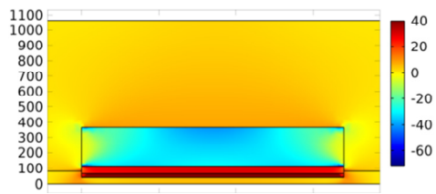
Fig 6.16 Cooling induced planar stress after cooling from 160°C to room temperature
