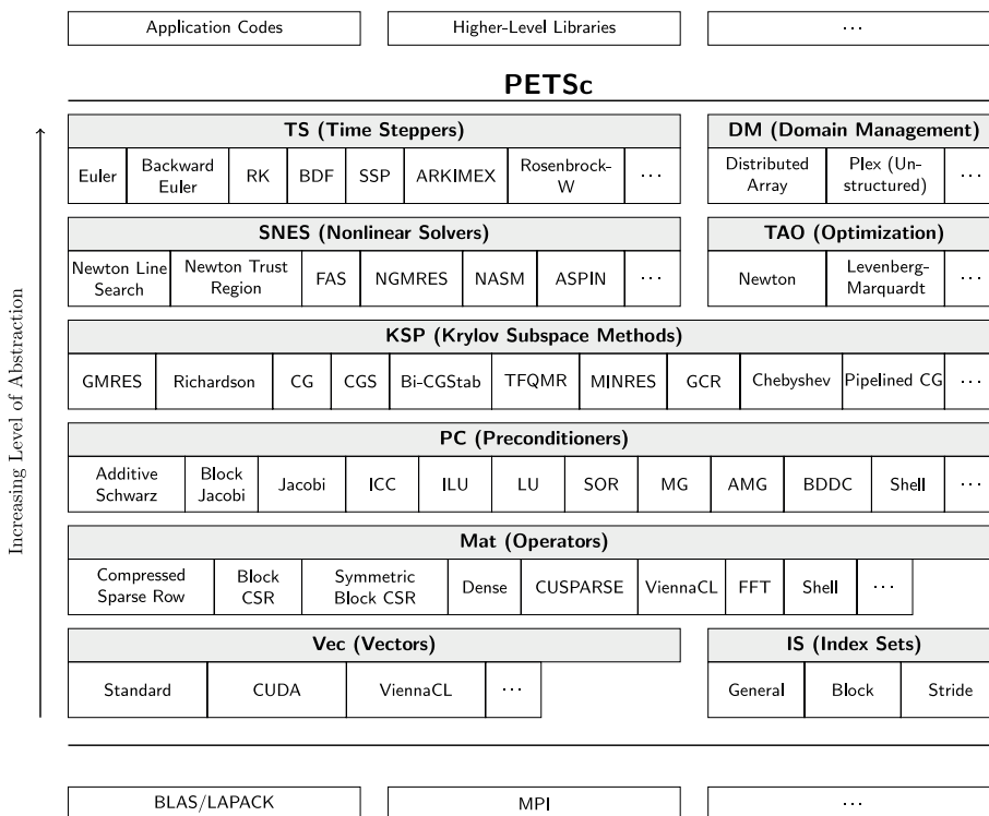
Figure 9.2: Petsc structure [54]
