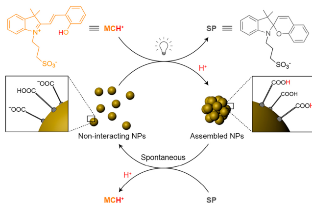
Figure 7. Visible-light-mediated assembly of gold nanoparticles functionalized with carboxylic-containing surface ligands dispersed in an aqueous medium operating under dissipative conditions. In the thermodynamic ground state, the colloids carry a net negative surface charge, safeguarding colloidal stability via electrostatic repulsion. Upon illumination with light, molecularly dissolved photoacids ( \text{MCH}^+ , orange) undergo a ring-closure reaction, thereby releasing protons ( \text{H}^+ ). The associated decrease in pH results in protonation of the surface-immobilized carboxylic acids. The diminished surface charge is no longer sufficient to ensure colloidal stability resulting in the formation of clusters. As the ring-closed reaction product (SP, gray) is metastable under the imposed reaction conditions, it slowly reverts back to its zwitterionic form. Upon doing so, protons are taken up from the dispersing medium. This leads to an increase in pH and a reinstatement of the surface charges on the colloids. On a mesoscopic scale, this results in disintegration of the particle clusters. Adapted from ref 22. Copyright 2016, John Wiley and Sons.
