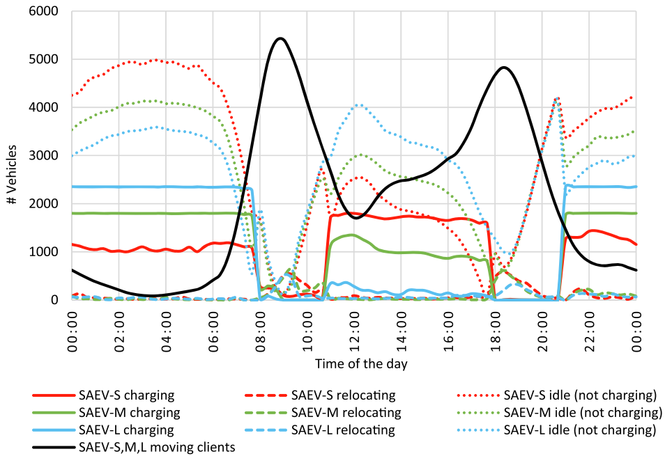
Fig. 9. State of the vehicles during the day for the scenarios where vehicles have 4-seats.
