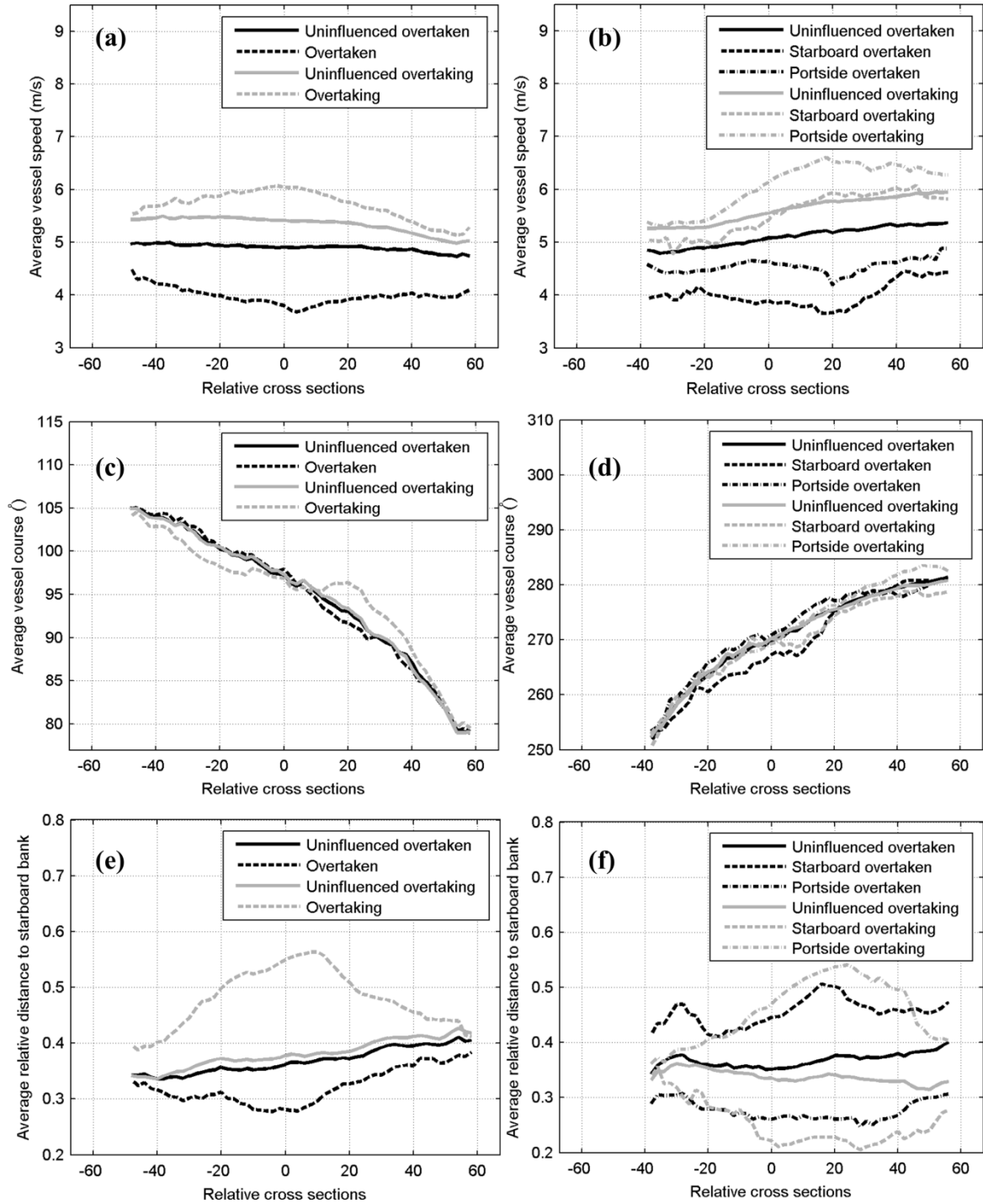
Fig. 11. Uninfluenced and influenced vessel speed (a), course (c) and distance to starboard bank (e) by overtaking encounters in Sea-Nieuwe Maas; uninfluenced and influenced vessel speed (b), course (d) and distance to starboard bank (f) by overtaking encounters in Nieuwe Maas-Sea.
