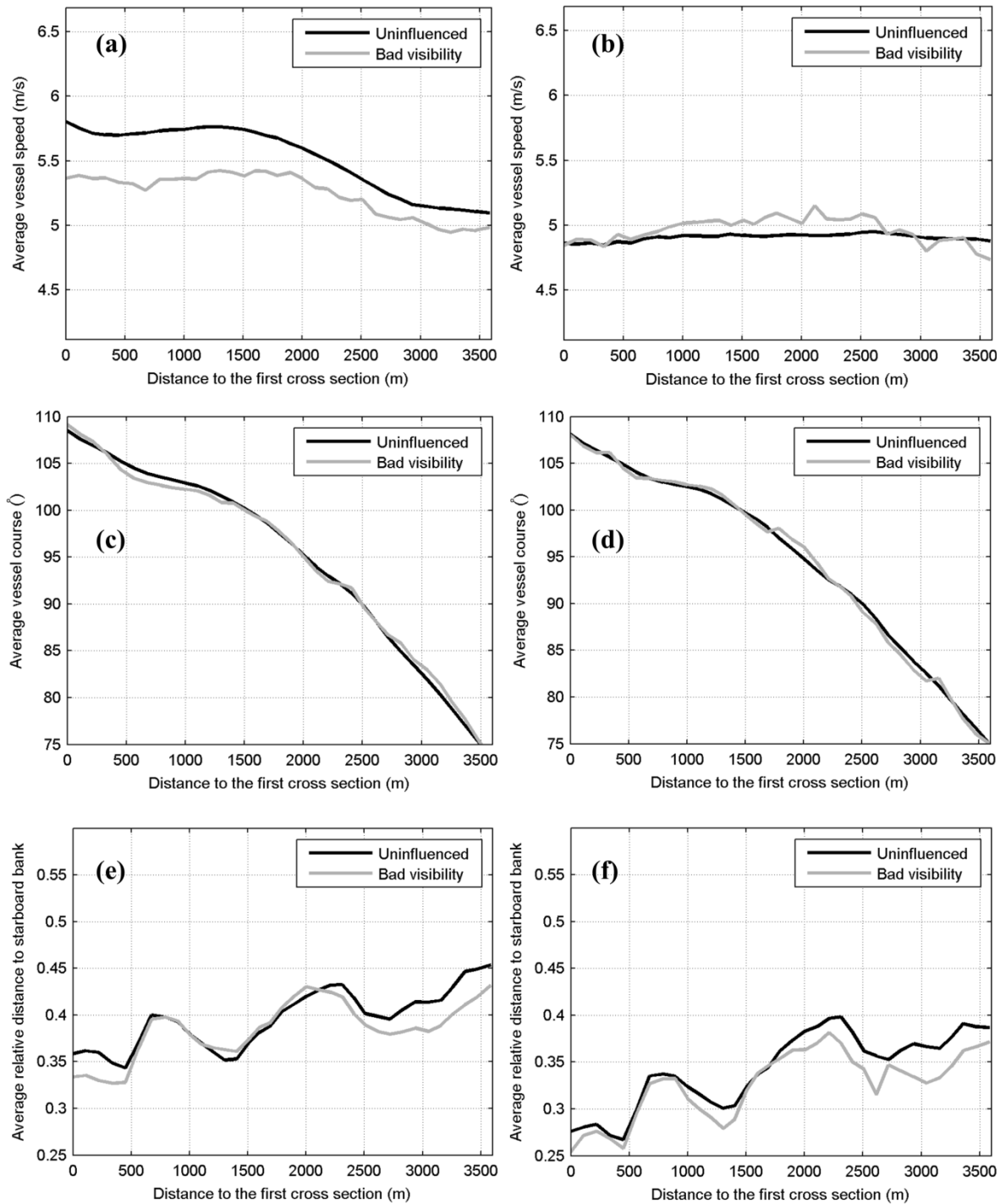
Fig. 7. Uninfluenced and influenced vessel speed (a), course (c) and distance to starboard bank (e) by visibility for container vessels in Sea-Nieuwe Maas; uninfluenced and influenced vessel speed (b), course (d) and distance to starboard bank (f) by visibility for GDC vessels in Sea-Nieuwe Maas.
