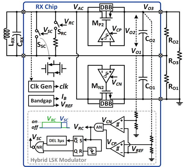
Fig. 4. System diagram of the single-stage triple-output RX with hybrid-LSK modulation.
