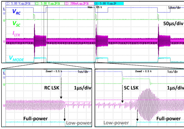
Fig. 9. Measured hybrid-LSK demodulation waveform of the proposed WPT system at V_{IN} = 3.3 V, D_{COIL} = 1 cm, and R_{O1} = R_{O2} = R_{O3} = 1 k \Omega .
