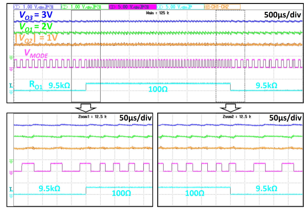
Fig. 8. Measured load-transient waveform of the proposed WPT system at V_{IN} = 3.3 \text{ V} , D_{COIL} = 1.5 \text{ cm} , and R_{O2} = R_{O3} = 1 \text{ k}\Omega .
