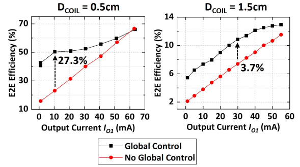
Fig. 11. Measured E2E power efficiency versus output current, I_{O1} , with or without global power regulation at V_{IN} = 3.3 V and I_{O2} = I_{O3} = 5 mA.
