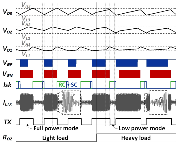
Fig. 3. Operational principle of the proposed WPT system achieving triple-output regulation under R_{O2} load transient.
