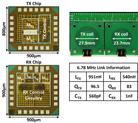
Fig. 6. Chip photos of the proposed TX and RX chips, and the 6.78-MHz inductive link information.
