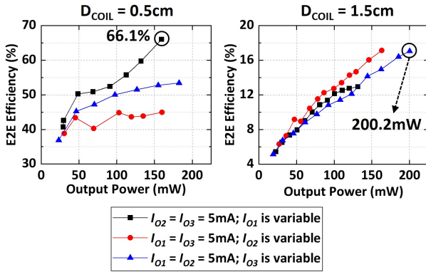
Fig. 10. Measured end-to-end (E2E) power efficiency of the proposed WPT system versus output power at V_{IN} = 3.3 V. I_{O1} , I_{O2} , and I_{O3} are the output currents flowing through R_{O1} , R_{O2} , and R_{O3} , respectively.
