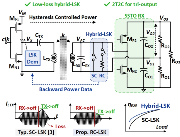
Fig. 2. Proposed WPT system with single-stage triple-output rectifier RX and fully integrated hybrid-LSK backscattering for global TX power regulation.
