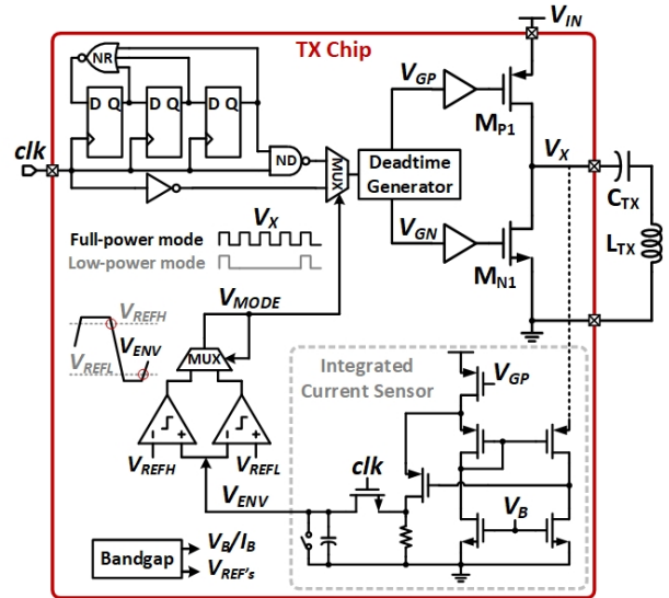
Fig. 5. System diagram of the class-D TX with global hysteresis power regulation based on hybrid-LSK demodulation.
