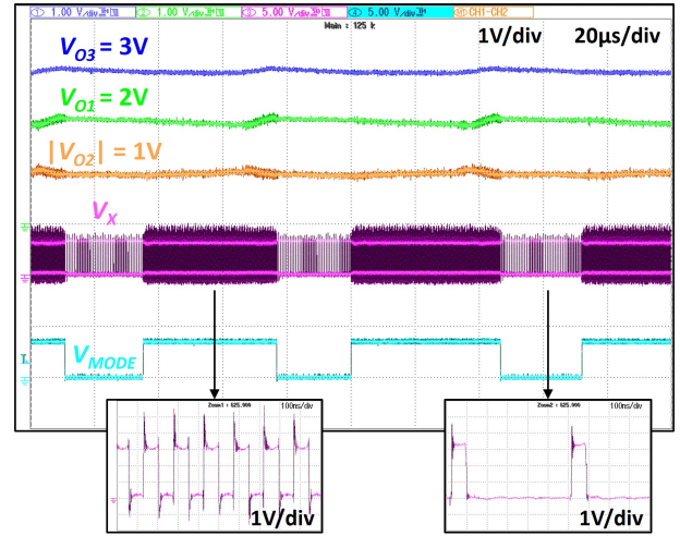
Fig. 7. Measured steady-state waveform of the proposed WPT system at V_{IN} = 3.3 \text{ V} , D_{COIL} = 1.5 \text{ cm} , and R_{O1} = R_{O2} = R_{O3} = 700 \Omega .
