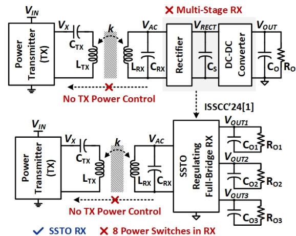
Fig. 1. Conventional wireless power transfer (WPT) system for biomedical devices (top), state-of-the-art triple-output WPT system (bottom).
