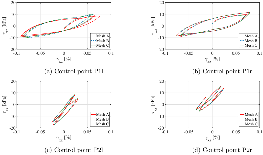
Figure 20: Domain size sensitivity analysis: \tau_{xz} - \gamma_{xz} cycles at the four control points in Figure 17b
