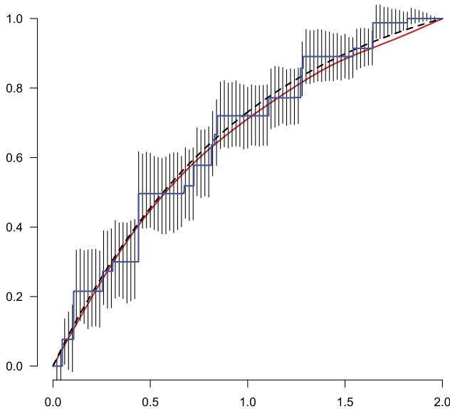
FIG. 11. Sen-Xu 95% confidence intervals for the (truncated exponential) distribution function F_0 , n = 1000 , observations are (T_i, \Delta_i) , where T_i is Uniform(0, 2) . Construction uses 1000 (smooth) bootstrap samples of indicators \Delta_i^* , using the SMLE (red) of the original sample. Dashed curve: truncated exponential distribution function.
