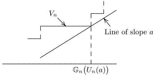
FIG. 6. The switch relation; G_n is the empirical distribution function of the T_i , V_n(t) = n^{-1} \Delta_i 1_{\{T_i \leq t\}} and U_n(a) = \operatorname{argmin}\{t : V_n(t) - aG_n(t)\} .
