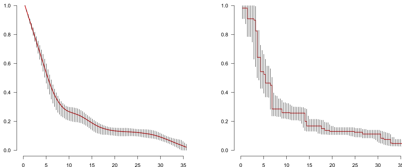
FIG. 5. Left: 95% confidence intervals, based on the SMLE, for the data in Slama et al. (2012), at the points 0.36, 0.72, . . . , 35.64. The bandwidth was determined by cross validation, both in the original sample and in the bootstrap samples. Right: Banerjee–Wellner type 95% confidence intervals, based on LR test for the (restricted) MLE’s, as proposed in Groeneboom and Jongbloed (2015).
