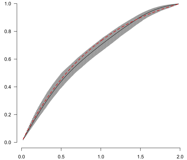
FIG. 12. 95% confidence intervals produced by the R package curstatCI for the (truncated exponential) distribution function F_0 , n = 1000 , observations are (T_i, \Delta_i) , where T_i is Uniform(0, 2) . The construction uses 1000 nonparametric bootstrap samples, as described in the text. The locally optimal bandwidth h (in principle different for each evaluation point) is also computed by a bootstrap experiment. Dashed curve: truncated exponential distribution function, solid curve: SMLE. A boundary correction is used in neighborhoods of 0 and 2.
