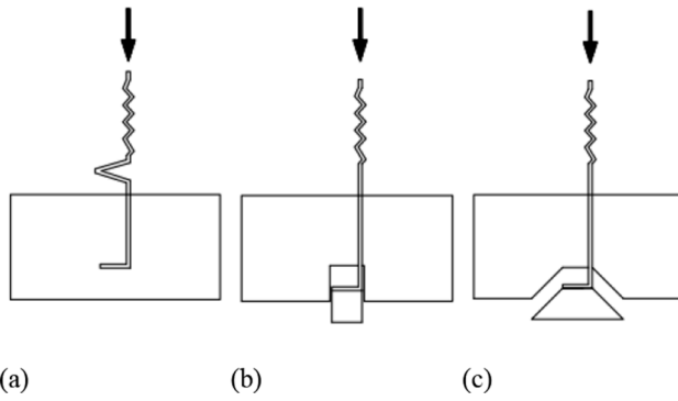
Fig. 4. Failure modes in Compression: Buckling failure(a), Piercing failure (b), Punching failure (c).
