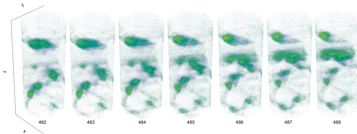
Fig. 15. Timeframes 482–488 of the bubbling fluidized bed using a superficial gas velocity of 17 cm/s. For this visualization we enhanced the images by postprocessing with a low-weight ( \lambda = 1/0.065 ) total variation filter.
