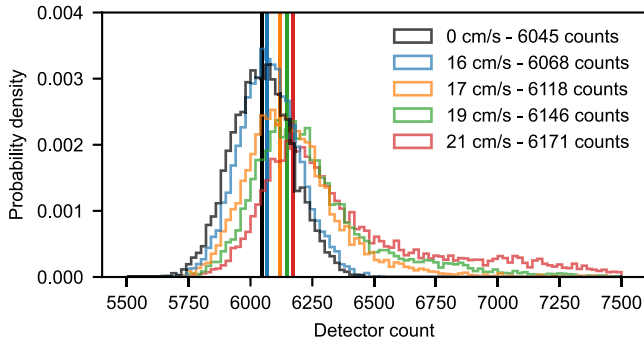
Fig. 4. Detector count statistics for 1000–1200 measurements of a central pixel, for different superficial gas velocities of a fluidized bed. Vertical lines indicate the modes.
