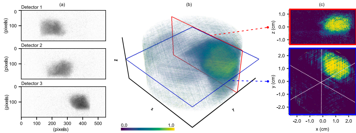
Fig. 12. A solitary bubble that is extracted from frame 475 of the Geldart B fluidized bed reconstruction with a superficial gas velocity of 17 cm/s. The visualization format is explained in Section 4.3.
