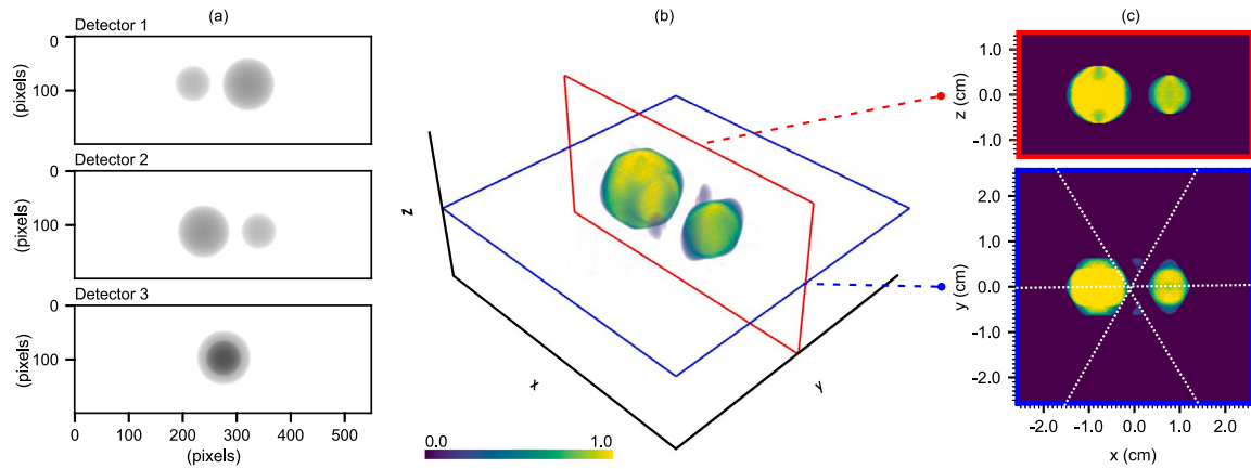
Fig. 7. Reconstruction of two simulated bubbles with diameters D_1 \approx 1.23 cm and D_2 \approx 0.83 cm (74 and 50 voxels, respectively), for which the projections overlap on Detector 3. The visualization format is explained in Section 4.3.
