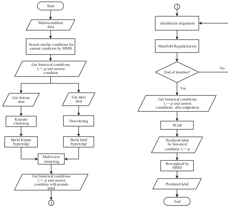
Fig. 3. Flow chart of DASP.
