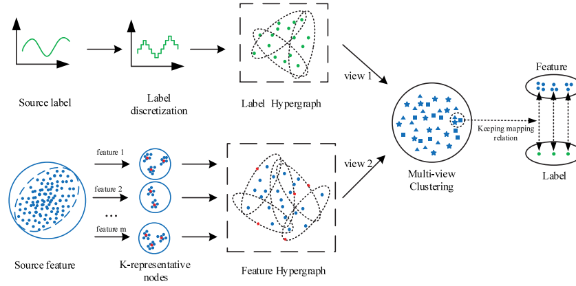
Fig. 2. Schematic diagram of pseudo label structure.
