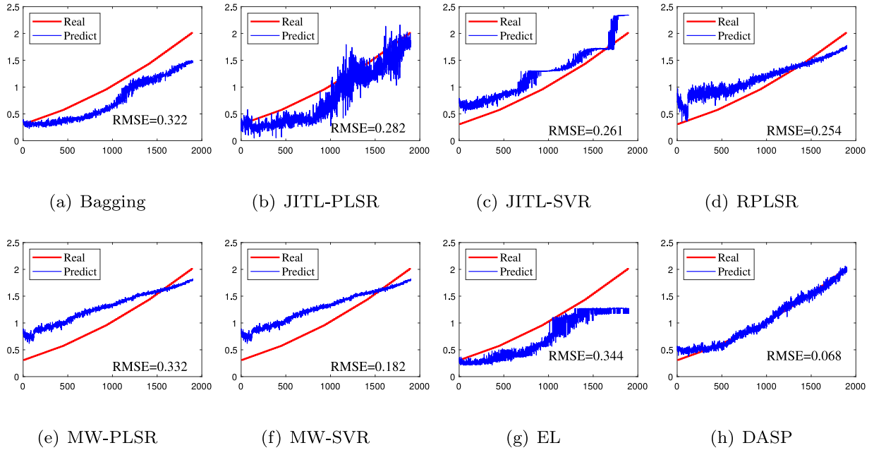
Fig. 10. MBVR prediction results of ball mill.
