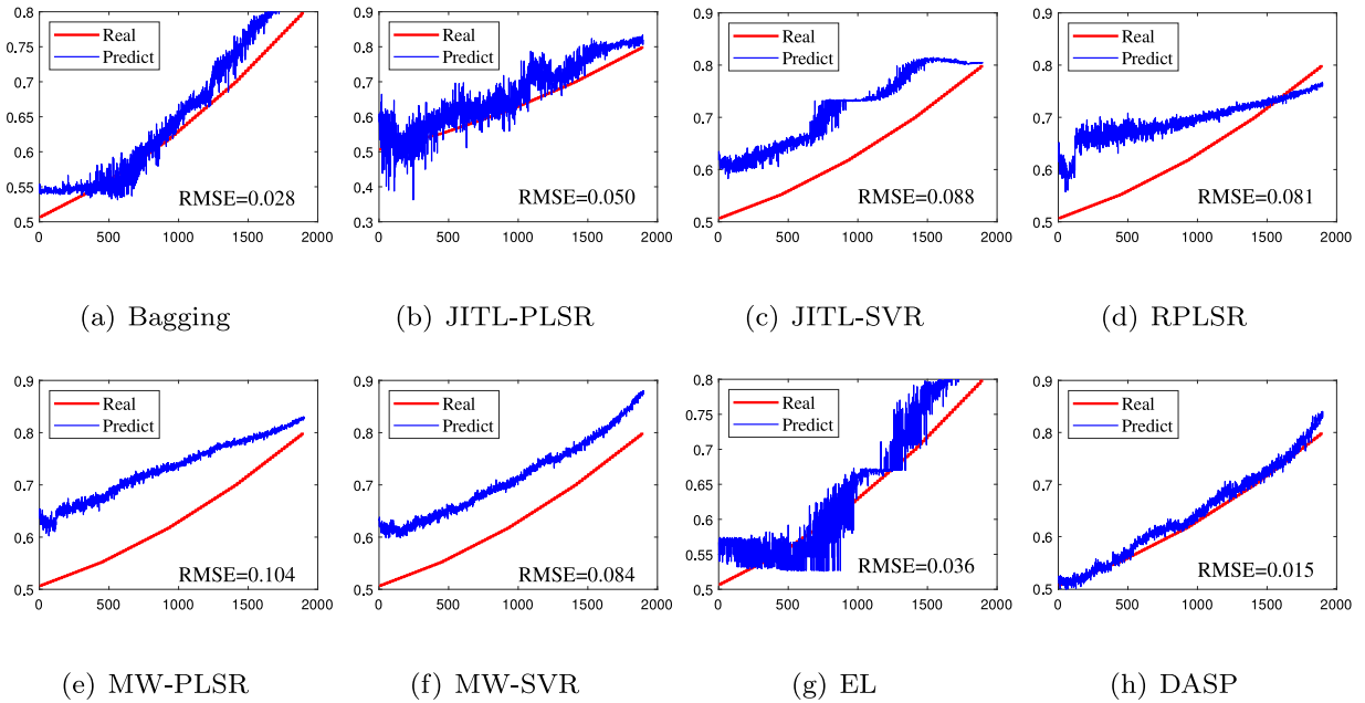
Fig. 12. CVR prediction results of ball mill.
