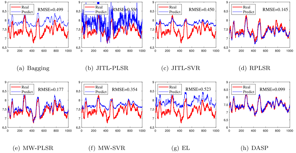
Fig. 9. TE component G prediction results.
