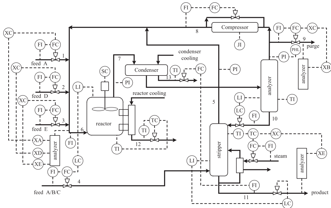
Fig. 4. Schematic diagram of TE process.
