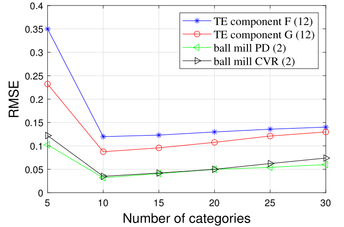
Fig. 15. Number of categories analysis.
