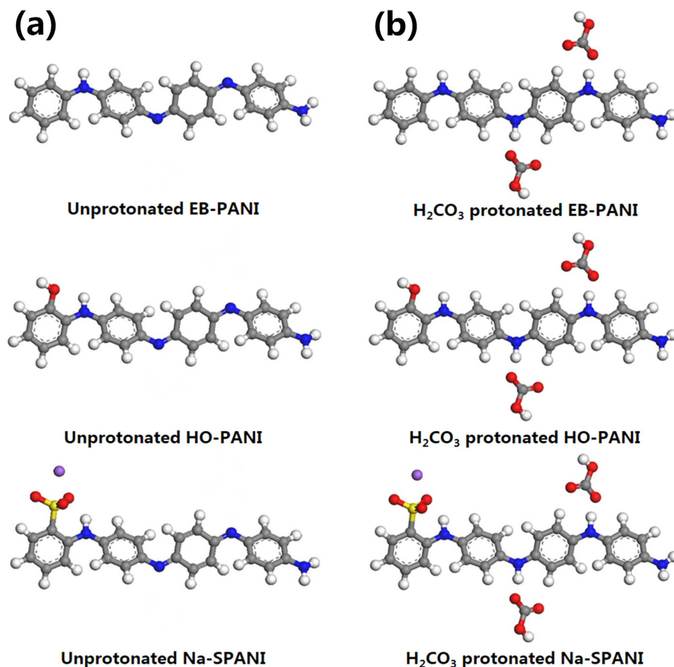
Figure 1. The finite molecular models with one polymer monomer for EB-PANI, HO-PANI and Na-SPANI: (a) Unprotonated and (b) \text{H}_2\text{CO}_3 -protonated states. The hydrogen, carbon, nitrogen, oxygen, sulfur and sodium atoms are shown in white, grey, blue, red, yellow and violet, respectively.
