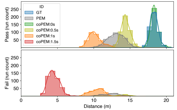
Fig. 6: Summarized results from 3000 runs (500 for each Perception Configuration). For each run, we consider a datapoint, i.e., the distance between the AV and the pedestrian at the moment of detection of the potential collision.
