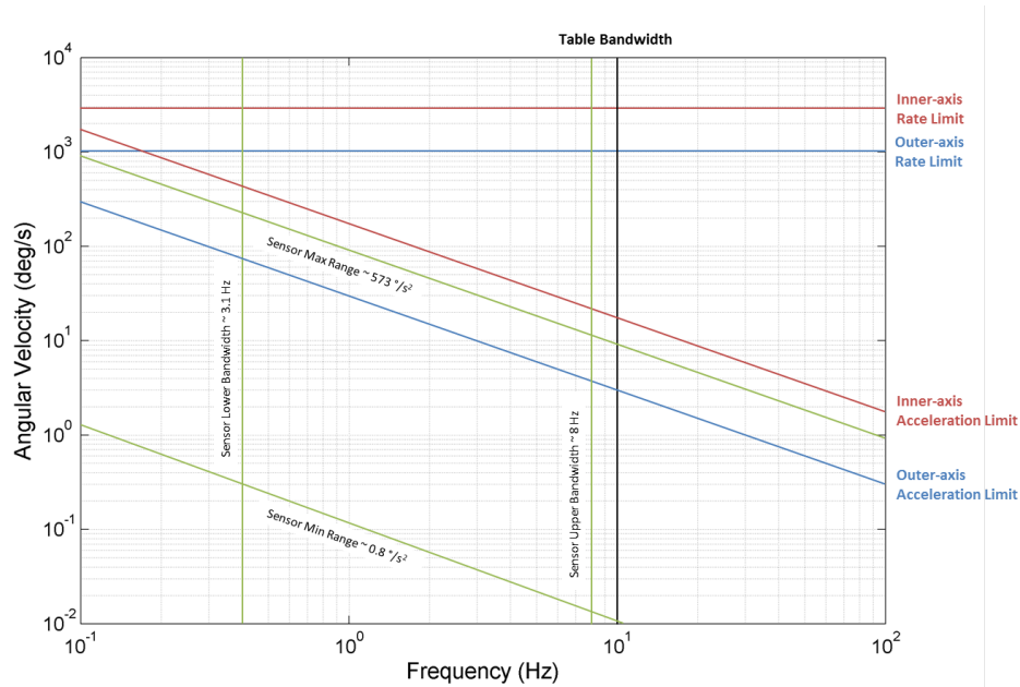
Figure 6. Motion simulator inner and outer-axis performance limitations and AA range.
