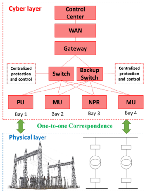
Figure 2.2 The Substation Communication Hybrid Architecture (NPR: Numerical Protection Relay, MU: Merging Unit, PU: Process Unit).
