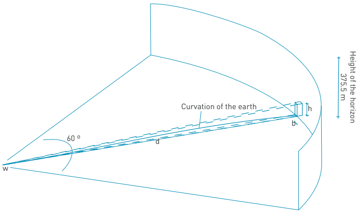
Figure 5 Model of the horizon impact percentage measurement method
