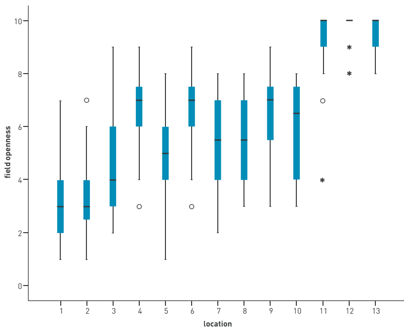
Figure 2 Box plots of rating of field openness by 32 participants for 13 locations. An increasing location number (x-axis) corresponds with and increasing isovist value
