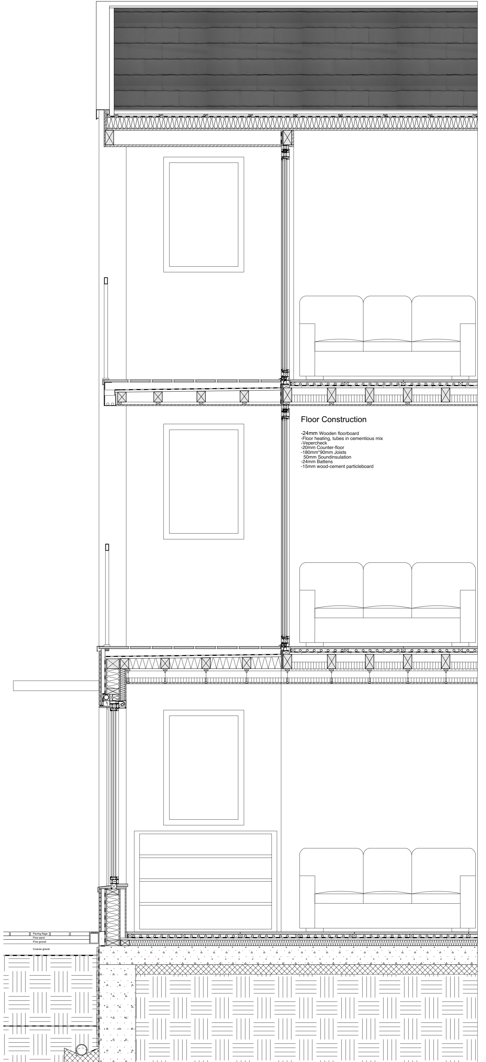
Section B-B 1:20
