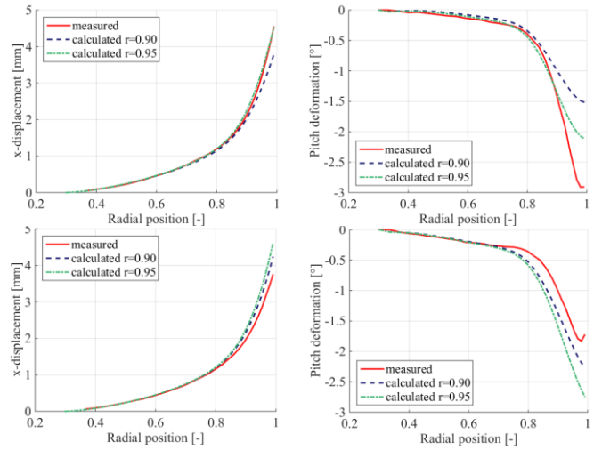
Figure 10: Bending (left) and pitch (right) deformations of the epoxy propeller, blade 1, obtained for measurement A (top) and B (bottom).
