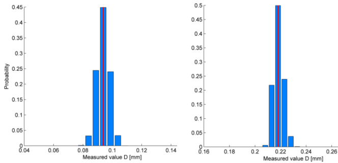
Figure 9: Distribution of measured displacements over the flat plate for tunnel speeds 4m/s (left) and 6m/s (right).
