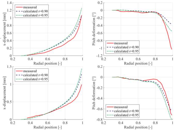
Figure 11: Bending (left) and pitch (right) deformations of the epoxy propeller, blade 1, obtained for measurement C (top) and D (bottom).
