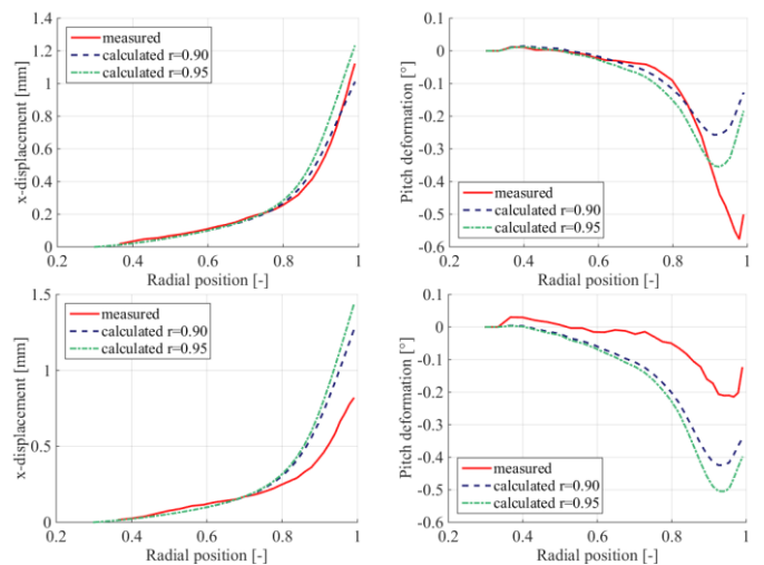
Figure 12: Bending (left) and pitch (right) deformations of the epoxy propeller, blade 2, obtained for measurement E (top) and F (bottom).
