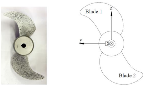
Figure 1: Picture of one of the small scale propellers and definition of the propeller coordinate system.
