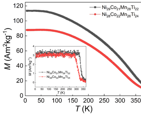
Fig. 5. Isofield M - T curves at 1 T for the \text{Ni}_{29}\text{Co}_{21}\text{Mn}_{28}\text{Ti}_{22} and \text{Ni}_{28}\text{Co}_{22}\text{Mn}_{26}\text{Ti}_{24} samples. The inset corresponds to the M - T curves at 0.01 T for these two alloys.
