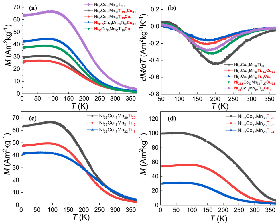
Fig. 3. (a) Isofield M - T curves at 1 T for \text{Ni}_{37-y}\text{Co}_{13}\text{Mn}_{30}\text{Ti}_{20-x}\text{Cu}_{xy} ( x, y = 0, 0.5, 1 ) series samples. (b) Relationship between dM/dT and temperature for the Cu-doped samples. (c) Isofield M - T curves at 1 T for \text{Ni}_{37}\text{Co}_{13}\text{Mn}_{30+x}\text{Ti}_{20-x} ( x = 0, 1, 2 ) samples. (d) Isofield M - T curves at 1 T for \text{Ni}_{33}\text{Co}_{17}\text{Mn}_{30-x}\text{Ti}_{20+x} ( x = 0, 2, 4 ) samples.
