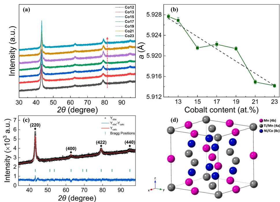
Fig. 1. (a) Room-temperature XRD patterns for \text{Ni}_{50-x}\text{Co}_x\text{Mn}_{30}\text{Ti}_{20} ( x = 12, 13, 15, 17, 19, 21, 23 ) alloys with different Co concentrations. (b) Lattice parameter a derived from the XRD refinement results as a function of the Co concentration for the \text{Ni}_{50-x}\text{Co}_x\text{Mn}_{30}\text{Ti}_{20} ( x = 12, 13, 15, 17, 19, 21, 23 ) alloys. (c) Room-temperature refined XRD measurement of the \text{Ni}_{33}\text{Co}_{17}\text{Mn}_{30}\text{Ti}_{20} sample. (d) Schematic crystal structures of B_2 austenite phase.
