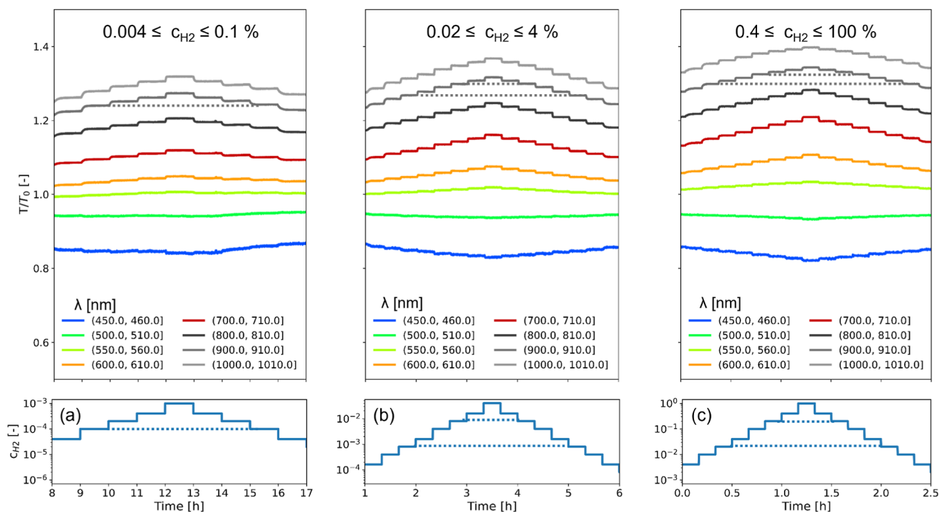
Figure 7. Optical transmission of a 40 nm \beta -Ta thin film capped by a 10 nm \text{Pd}_{0.6}\text{Au}_{0.4} capping layer relative to the transmission of the as-prepared film as a function of time during which the hydrogen concentration was stepwise changed in the regimes (a) 0.004 \leq c_{\text{H}_2} \leq 0.1\% , (b) 0.02 \leq c_{\text{H}_2} \leq 4\% , and (c) 0.4 \leq c_{\text{H}_2} \leq 100\% . The dashed lines indicate levels of the same transmission (top panel) and hydrogen concentration (bottom panel).
