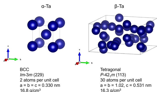
Figure 1. Unit cell and unit cell parameters of \alpha -Ta and \beta -Ta. Data on \alpha -Ta and \beta -Ta were adapted from refs 26 and 43, respectively. Visualizations are made with VESTA. 44
