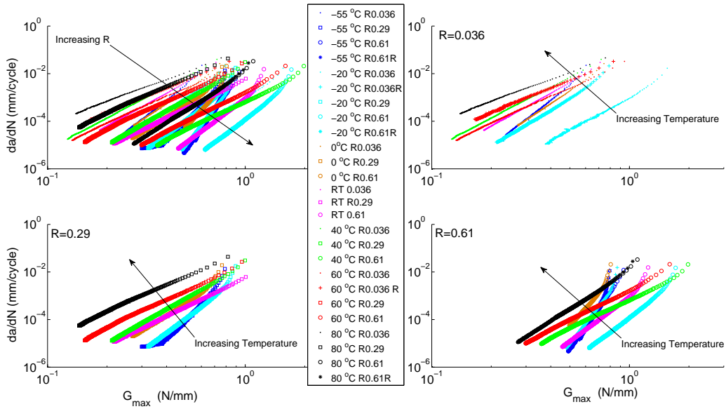
Figure 1: Crack growth rate as a function of G_{\max} . The top left panel shows the results for all experiments. The top right panel shows only the results for R=0.036 , the bottom left shows R = 0.29 , and the bottom right panel shows R = 0.61 . Increasing R (and keeping G_{\max} constant) resulted in a decrease of the crack growth rate. Conversely, an increase in temperature produced an increased crack growth rate.
