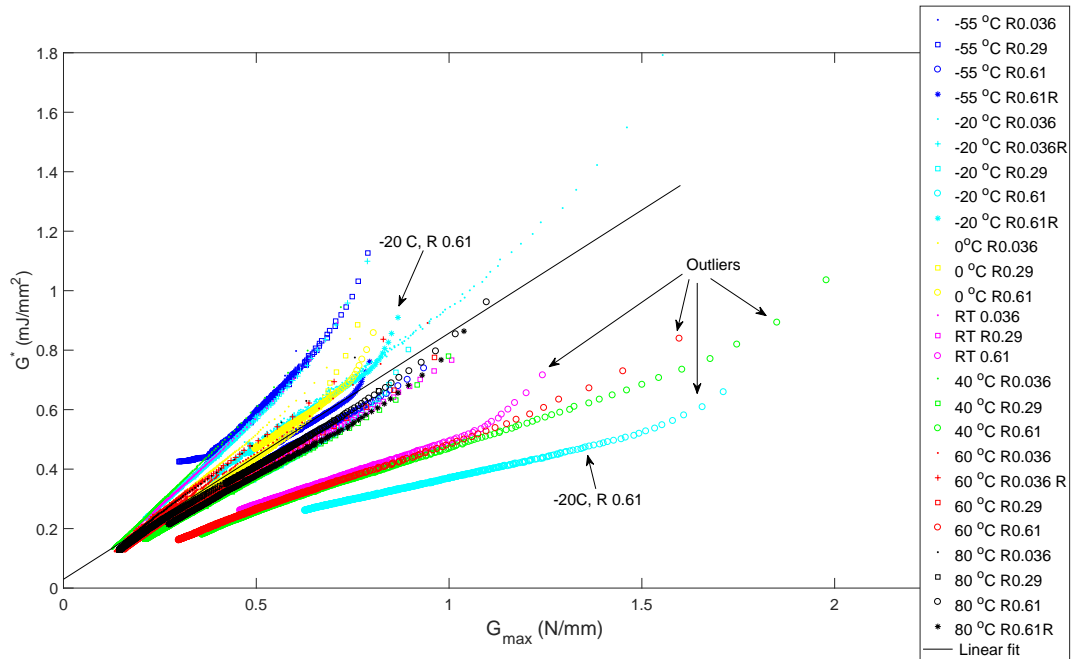
Figure 7: G^* as a function of G_{max} . Four tests show a different behaviour compared to the bulk of the data. These correspond to the four outliers marked in figure 6. A linear fit through the data is also shown ( R^2 = 0.8914 ). This fit excludes the four tests marked as outliers.
