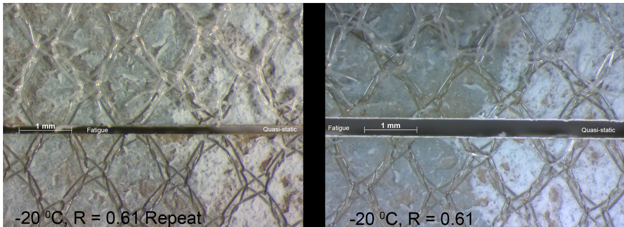
Figure 8: Image of the fracture surfaces of the two tests conducted at -20\text{ }^\circ\text{C} and R = 0.61 . The left panel shows the repeat test, and the right panel shows the first test. The first test (right panel) is one of the outliers identified in figures 6 and 7. The left panel corresponds to a test whose behaviour matched that of the bulk of the experiments. The direction of crack growth was from left to right. The images show the boundary between the end of the fatigue test (left), so low crack growth rate, and the quasi-static loading (right) used to generate a new pre-crack, or break open the specimen. Both the top and bottom fracture surfaces are shown, separated by a small gap.
