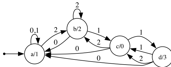
Figure 4: A 3-DFAO for the difference sequence A_{n+1} - 7n - 3 of the anti-Jacobsthals.
