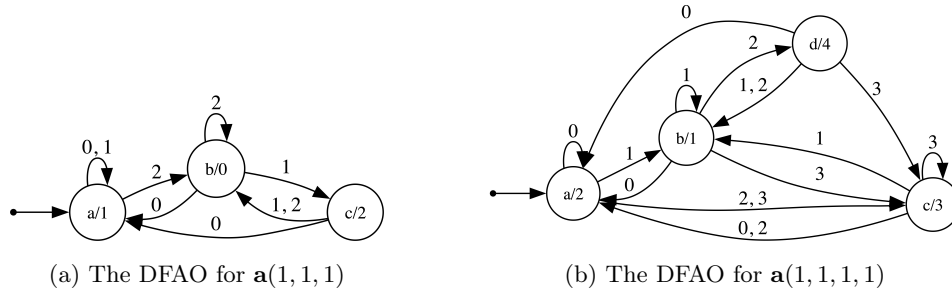
Figure 5: The 3-DFAO for the difference sequence A_{n+1} - 10n - 5 for the anti-Tribonacci sequence in (a) and A_{n+1} - 17n - 8 for the anti-Tetragonacci sequence in (b).
