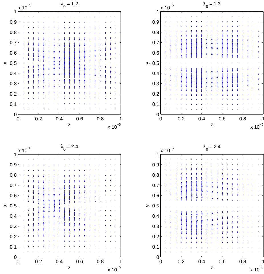
Figure 6.14: Velocity field in the xz - and yz -plane, through the focal point for \lambda_0 = 1.2\mu\text{m} and \lambda_0 = 2.4\mu\text{m} . Near the focal point we have a zero z component in all the plots. Also in the xz -plane we have the velocity pointing towards the central axis while in the yz -plane is it pointing away from the central axis.
