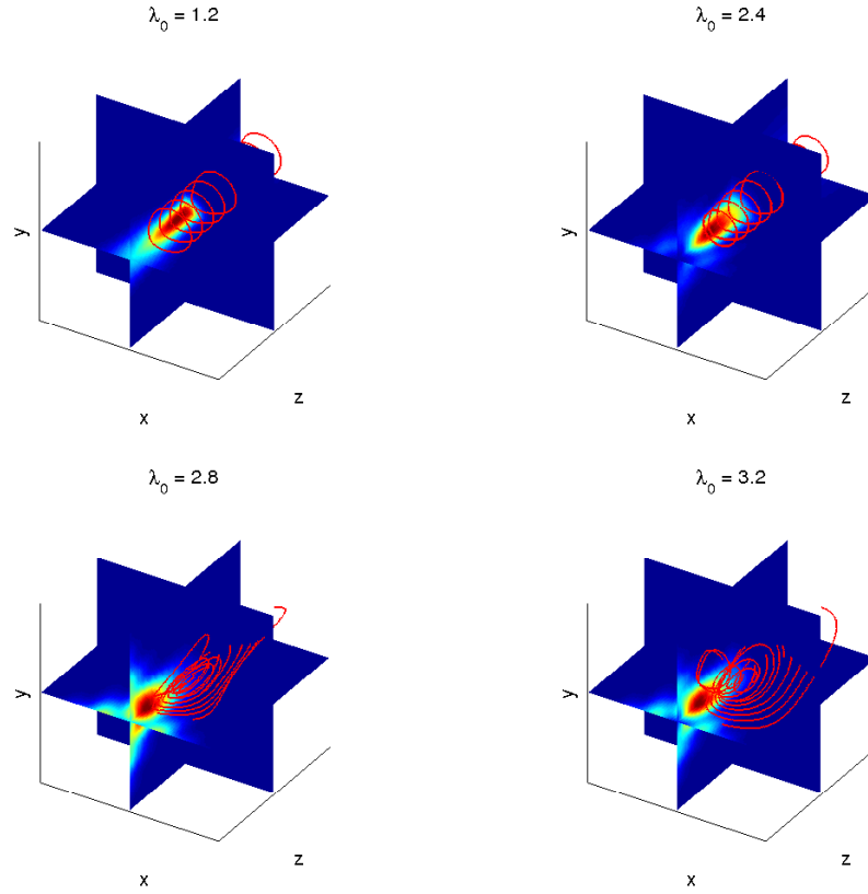
Figure 6.16: Velocity field in the xz - and yz -plane, through the focal point for \lambda_0 = 1.2\mu\text{m} and \lambda_0 = 2.4\mu\text{m} . Near the focal point we have a zero z component in all the plots. Also in the xz -plane we have the velocity pointing towards the central axis while in the yz -plane is it pointing away from the central axis, following our conjecture based on the force density.
