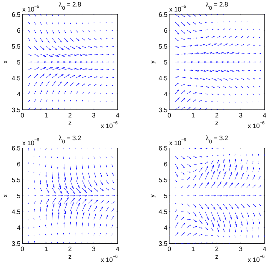
Figure 6.11: Force density in the xz - and yz -plane for \lambda_0 = 2.8 \mu\text{m} and \lambda_0 = 3.2 \mu\text{m} . For these wavelengths there is a significant z component of the force density, suggesting that the \mathbf{f}_{\text{dis}} term from (2.110) starts to contribute due to the relatively large values of \epsilon'' for these wavelengths.
