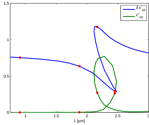
Figure 5.5: The permittivity of the wavelengths of interest as function of the fluid wavelengths, 0.91 \mu\text{m} , 1.88 \mu\text{m} , 2.45 \mu\text{m} and 2.17 \mu\text{m} respectively. We see that different vacuum wavelengths can have similar fluid wavelengths because of the index of refraction.
