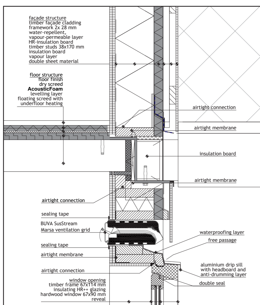
Detail 1
