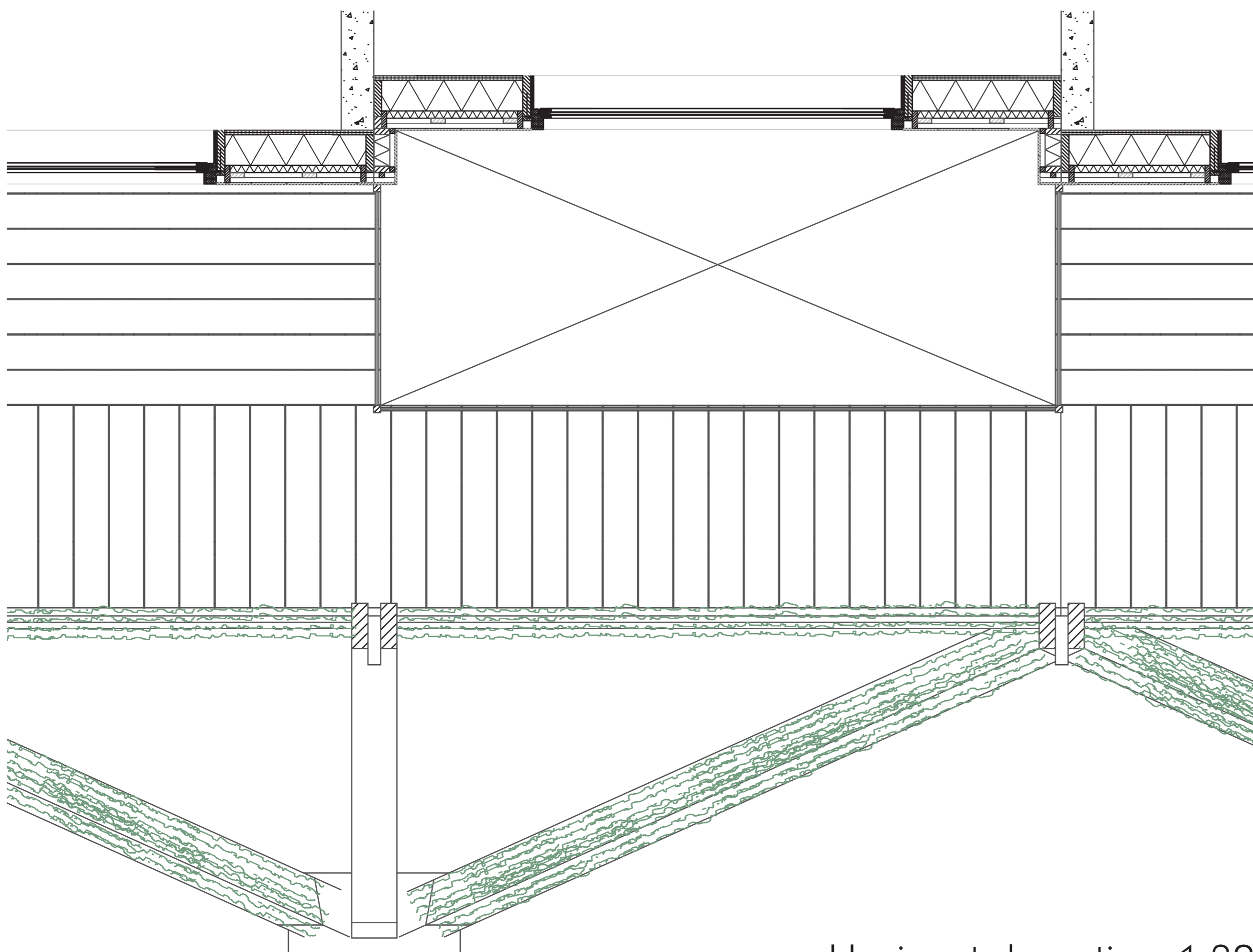
Horizontal section 1:20
