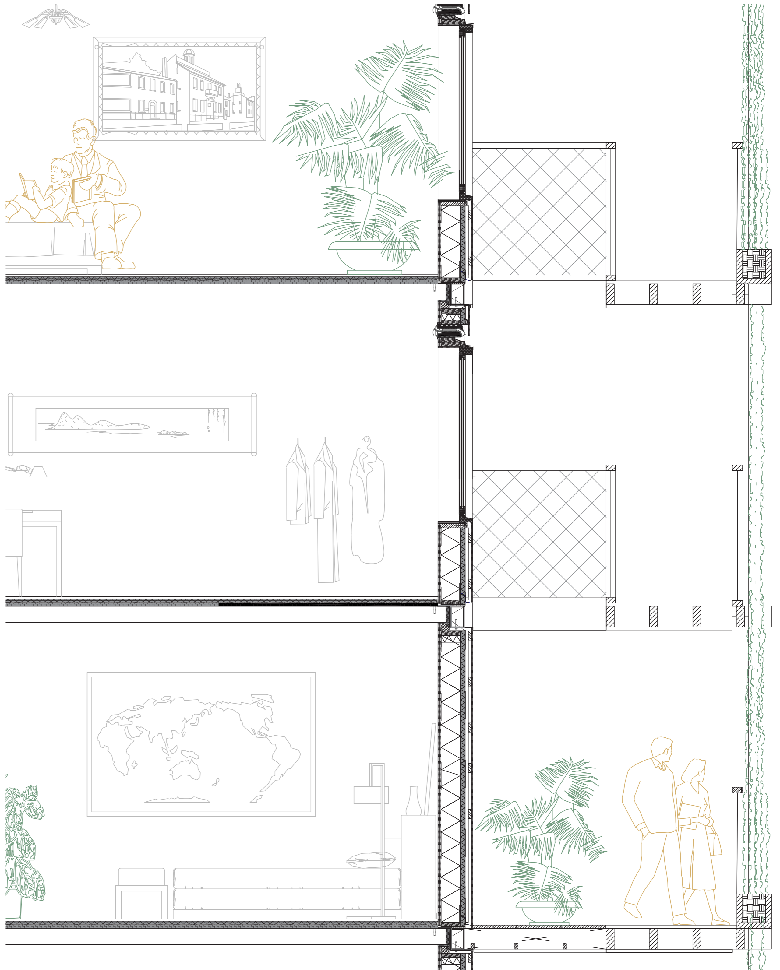
Vertical section 1:20
