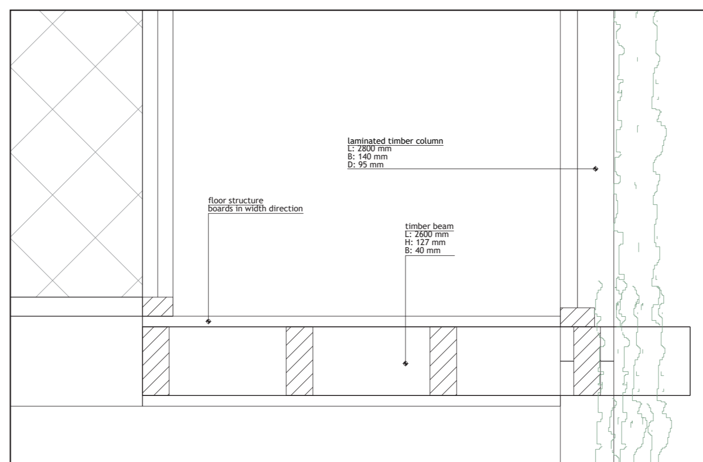
Detail 2
