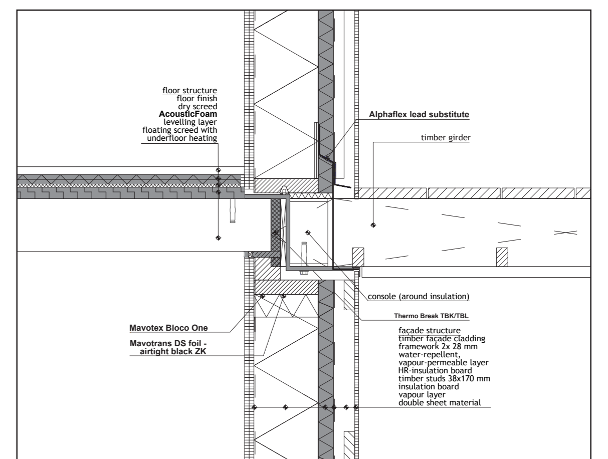
Detail 3
