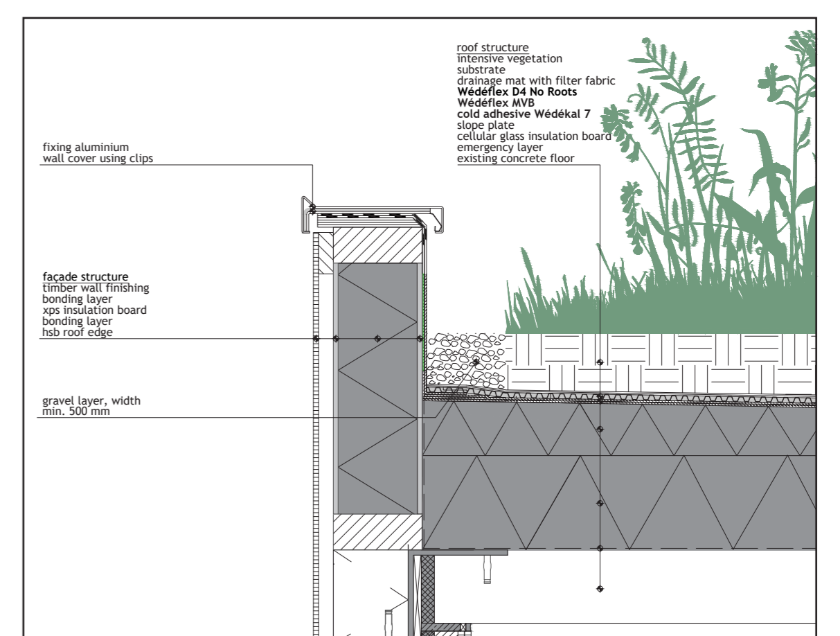
Detail 6
