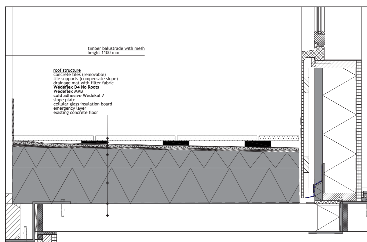
Detail 5
