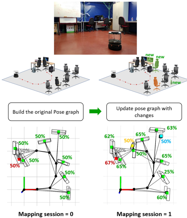
Fig. 1. Proof of concept of the dynamic mapping method in an indoor environment. First, the original object-based pose graph is built (7 chairs, 1 computer and 1 backpack were mapped). For the adaptation of the map, one chair was moved and a bottle and a screen were added. The map adapted to the changes adding the new objects and increasing or decreasing the probabilities of the old ones.
