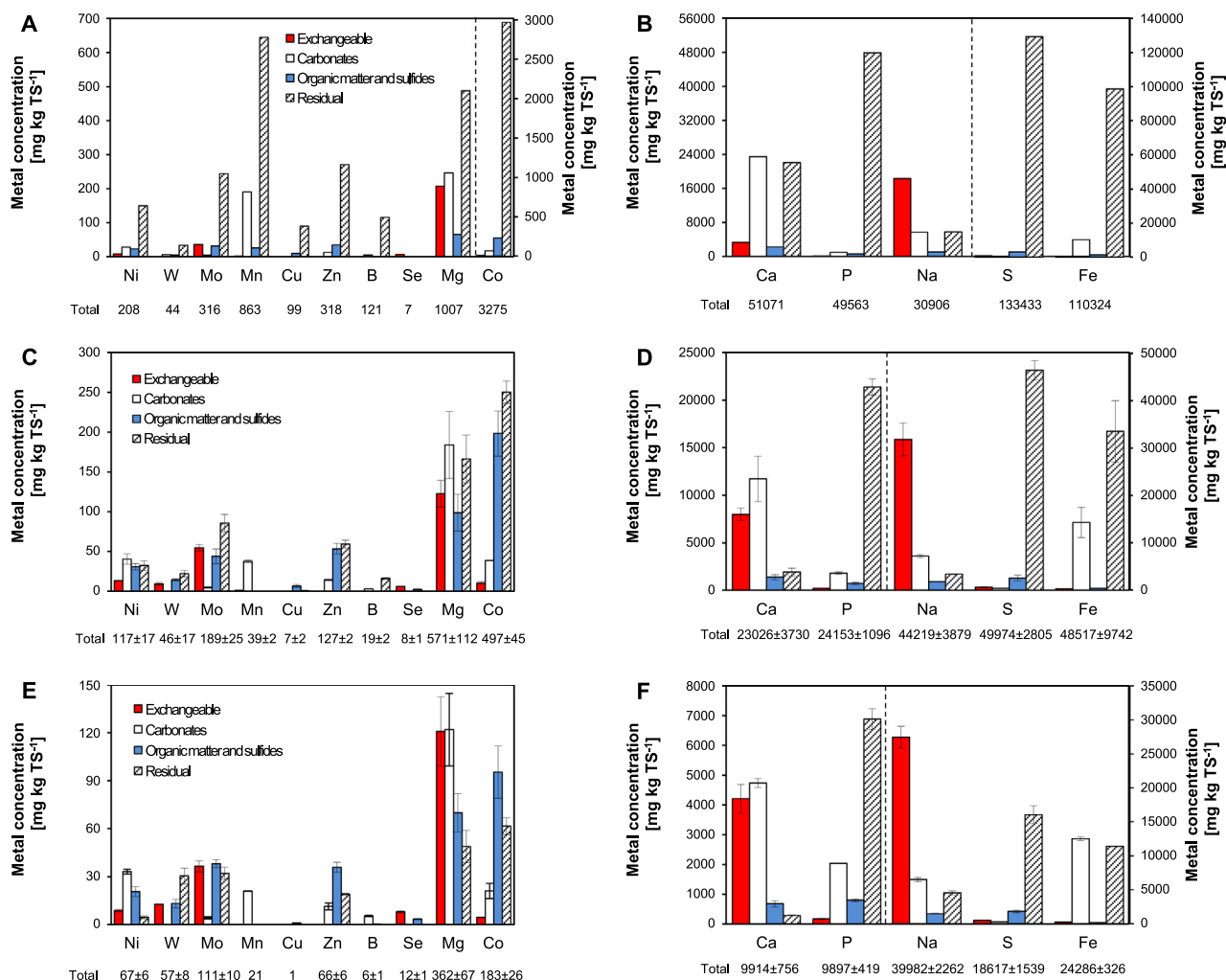
Fig. 5. Trace and macro elements concentration [ \text{mg kg TS}^{-1} ], and partitioning in the operationally defined fractions after one month of operation. A, B. Inoculum biomass. C, D. AnMBR1. E, F. AnMBR2. After dashed line the elements concentration must be read from the secondary y-axis.
