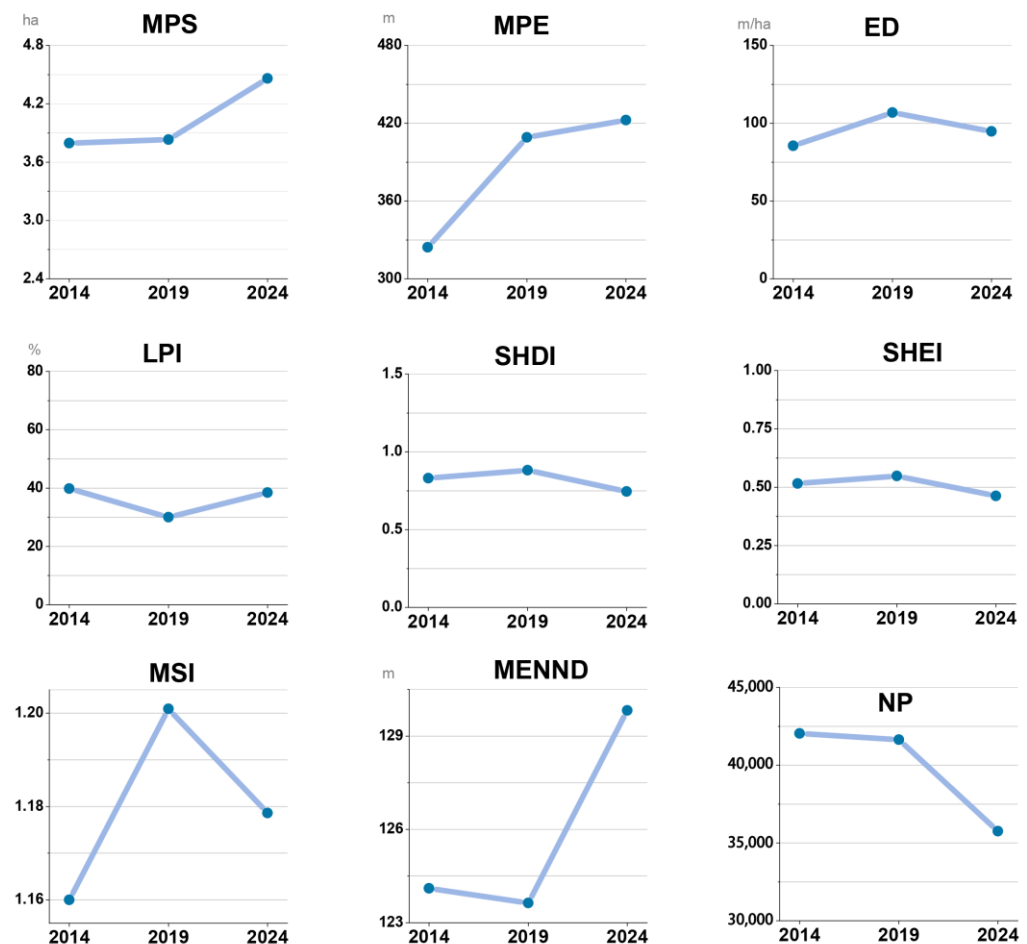
Figure 8. The evolution of spatial indicators at the landscape level from 2014 to 2019 to 2024. MPS: Mean patch size (ha); MPE: Mean patch edge (m); ED: Edge density (m/ha); LPI: Largest patch index (%); SHDI: Shannon's diversity index; SHEI: Shannon's evenness index; MSI: Mean shape index; MENND: Mean Euclidean nearest neighbor distance (m); NP: Number of patches.
