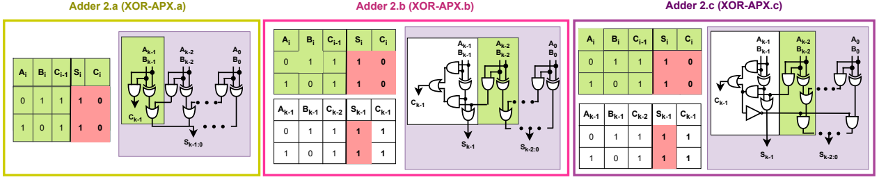
Fig. 4. XOR-based Approximate Adder Designs.
