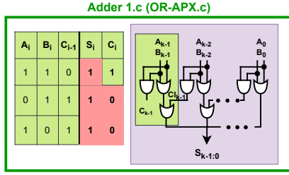
Fig. 3. OR-based Approximate Adder Design
