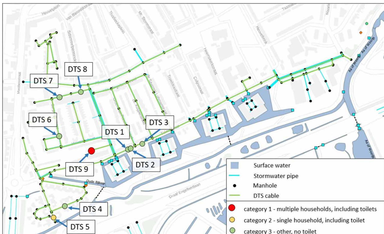
Figure 2 | Results of DTS monitoring with categorization of illicit connections.
